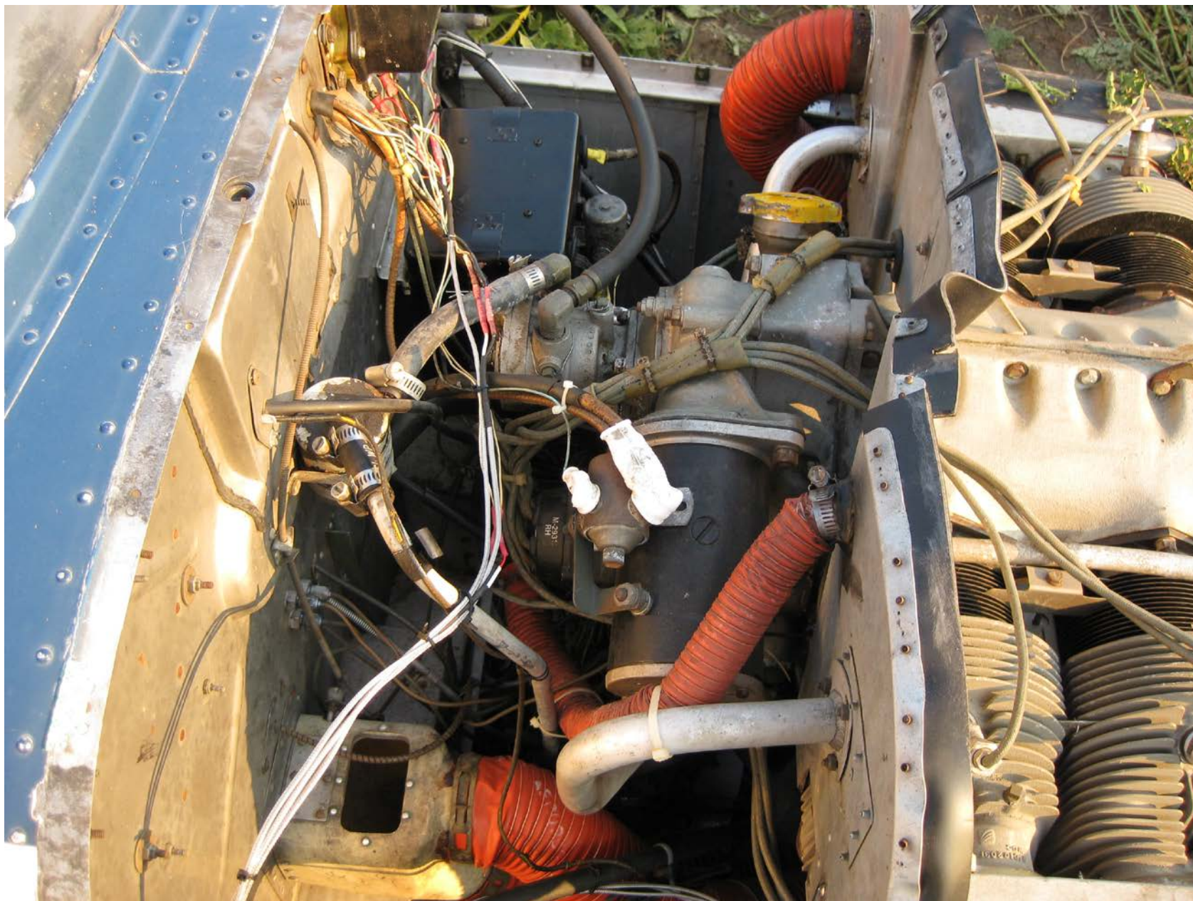
Photo 5 – View of the top rear engine compartment (courtesy of the Federal Aviation Administration).
