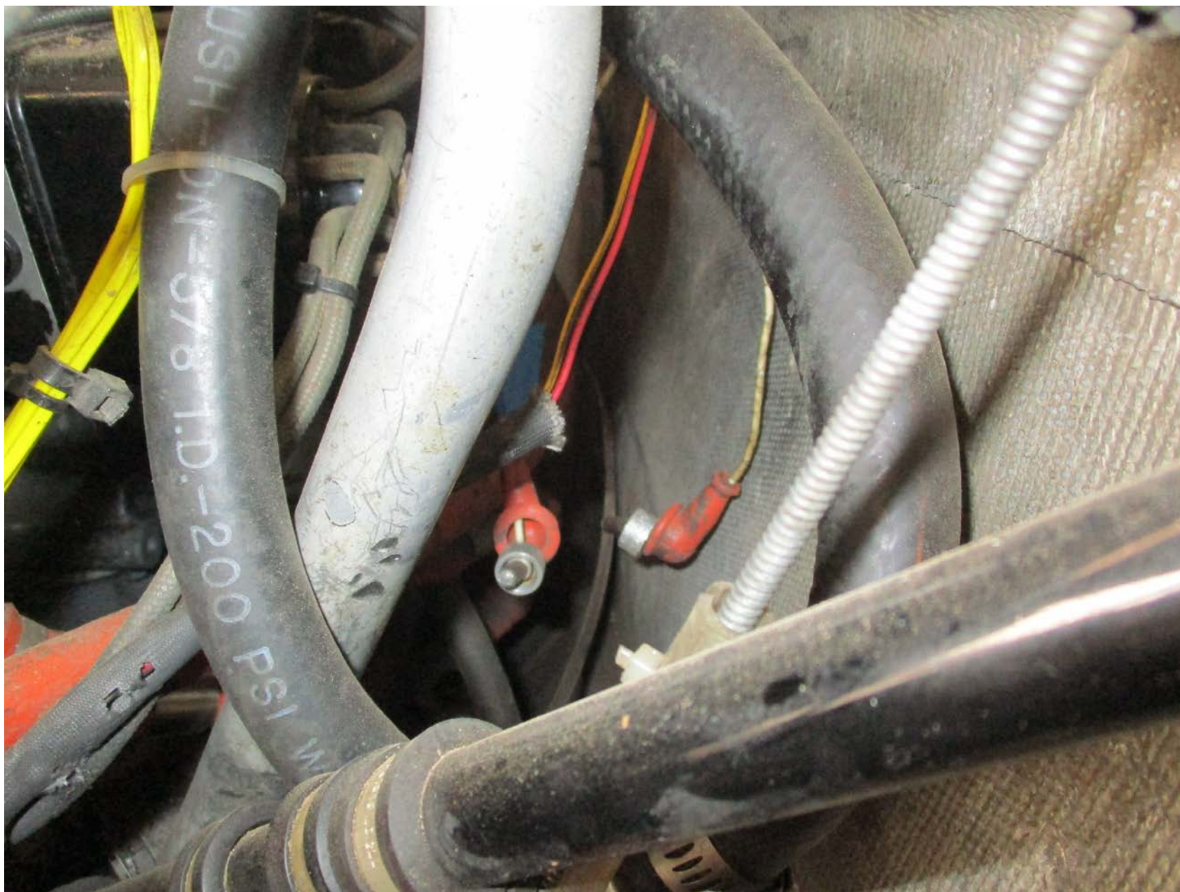
Photo 5 – Magneto primary leads
