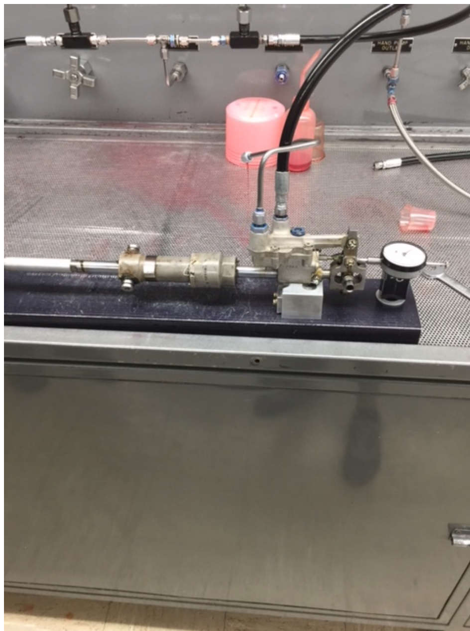
Photo 7 – View of the tail rotor servo being bench tested (courtesy of Helicopter Accessory Service Inc.).
