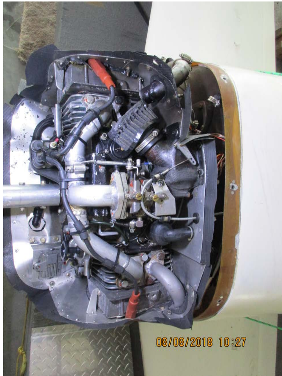
Photo 7 - FAA supplied overhead photo of the engine.
