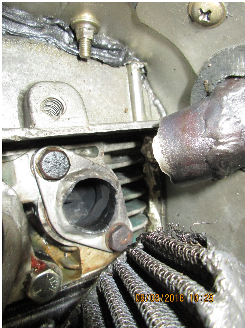
Photo 8 - FAA supplied close up photo of a separation in an exhaust pipe.
