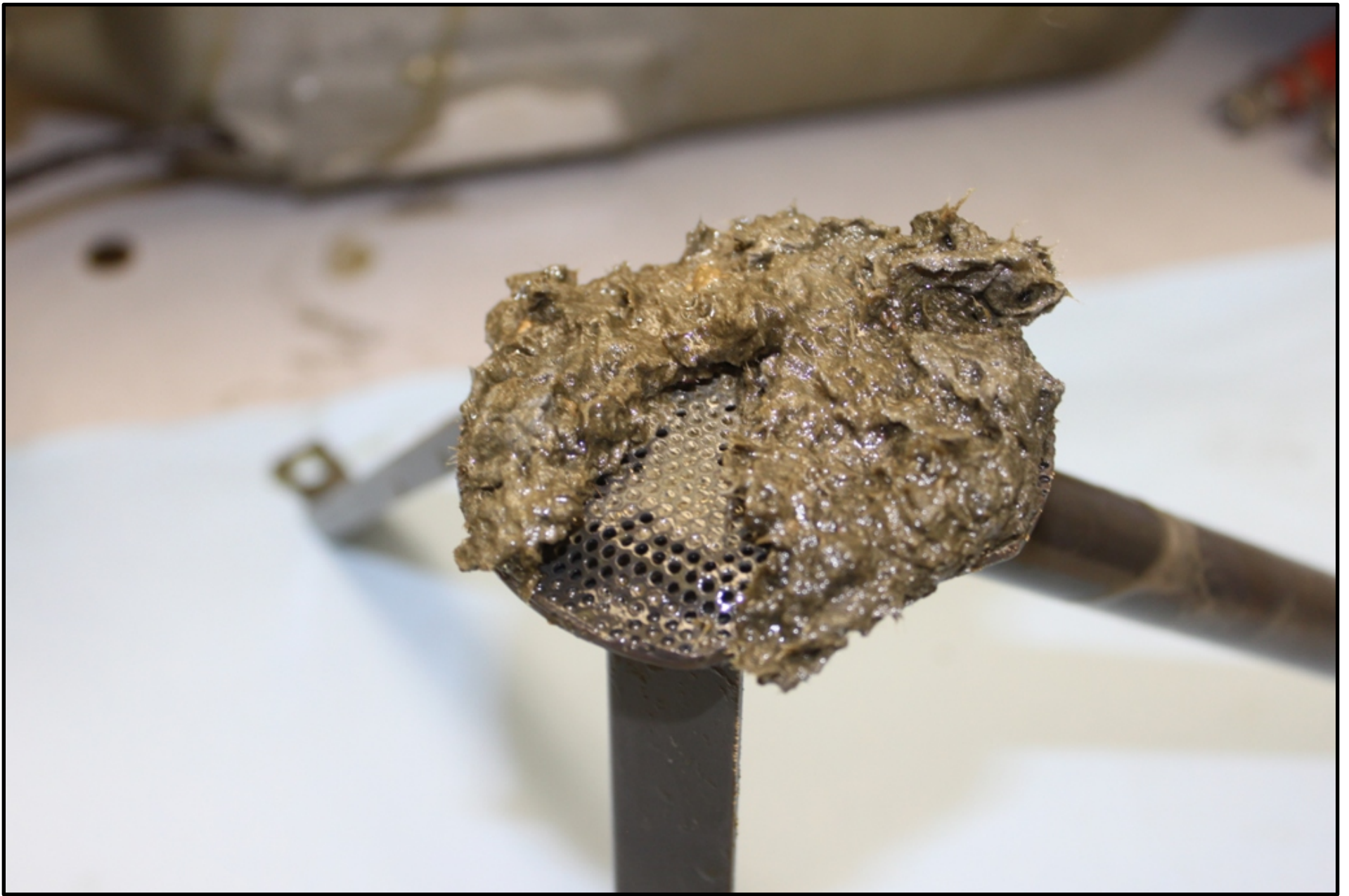
Photo 7 – Engine Oil Sump Pickup Screen
