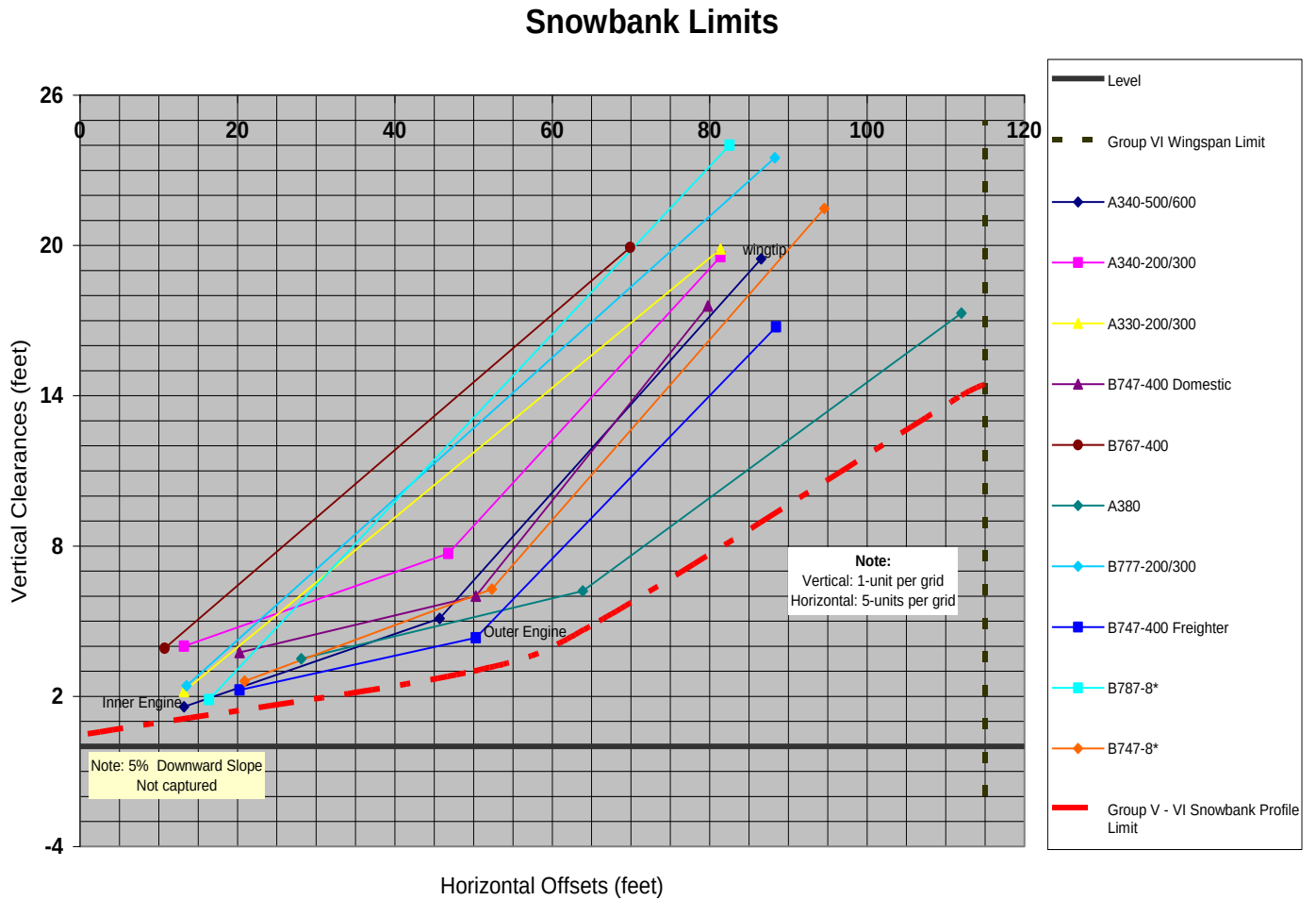
Figure B-2. Individual Height Profiles of Airplane Wingtips and Outer and Inner Engine Nacelles' Lower Edges for Airplane Design Groups V and VI (* indicates preliminary data)
