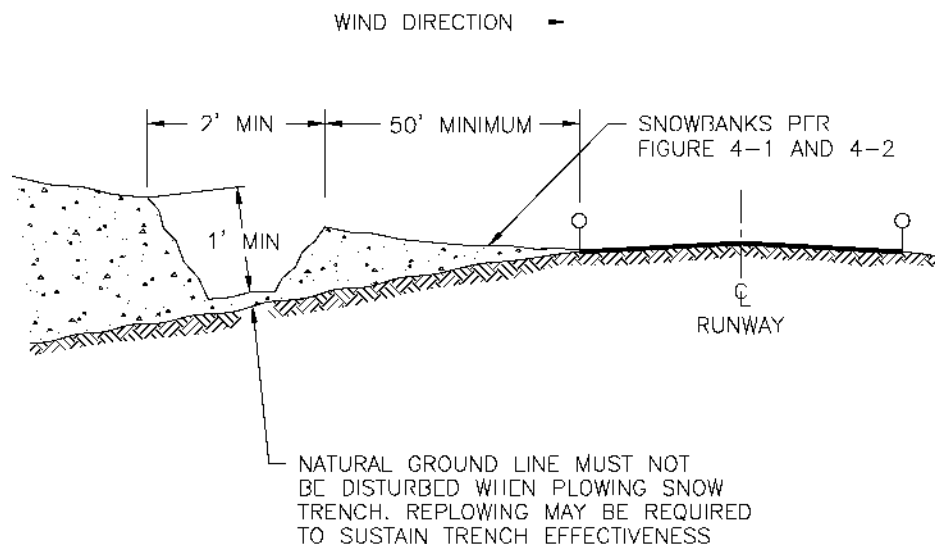
Figure 4-6. Typical Snow Trench Dimensions
