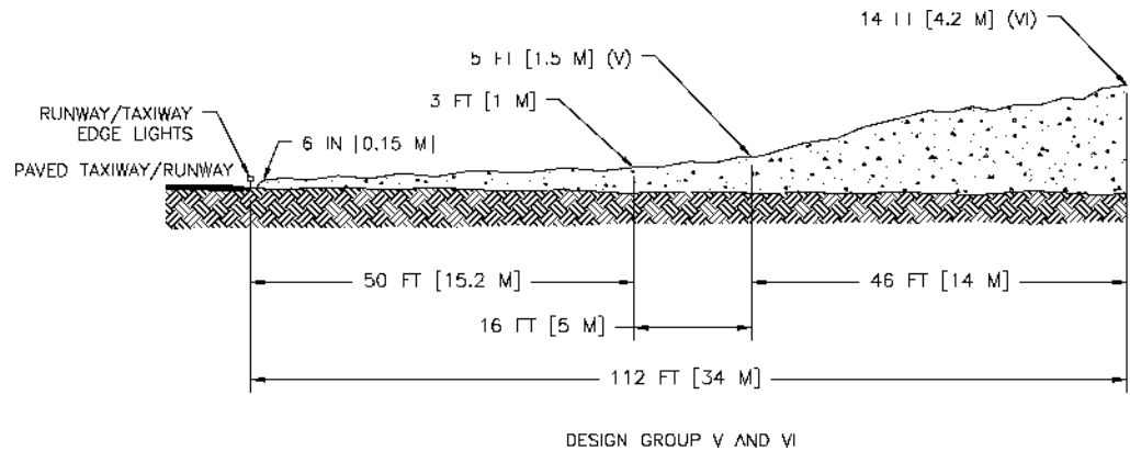
Figure 4-1. Snow Bank Profile Limits Along Edges of Runways and Taxiways with the Airplane Wheels on Full Strength Pavement (see Figure 4-2 guidance)
