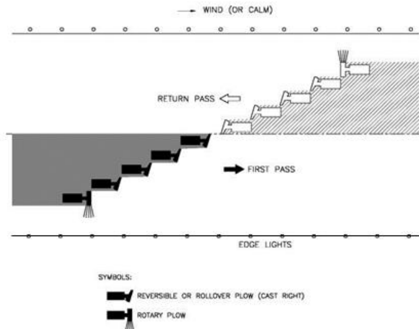
Figure 4-4. Possible Team Configuration During Light Snowfall with Parallel or Calm Wind
