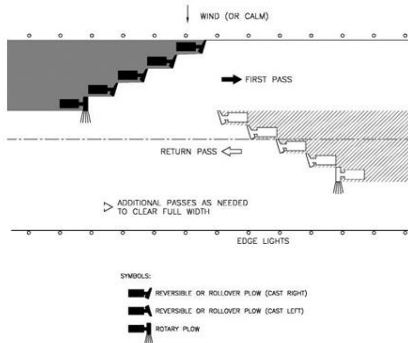
Figure 4-3. Possible Team Configuration with Perpendicular Wind
