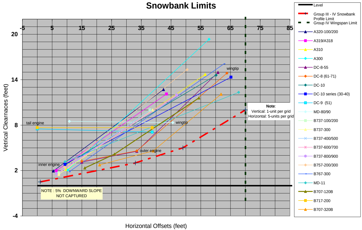
Figure B-1. Individual Height Profiles of Airplane Wingtips and Outer and Inner Engine Nacelles' Lower Edges for Airplane Design Groups III and IV
