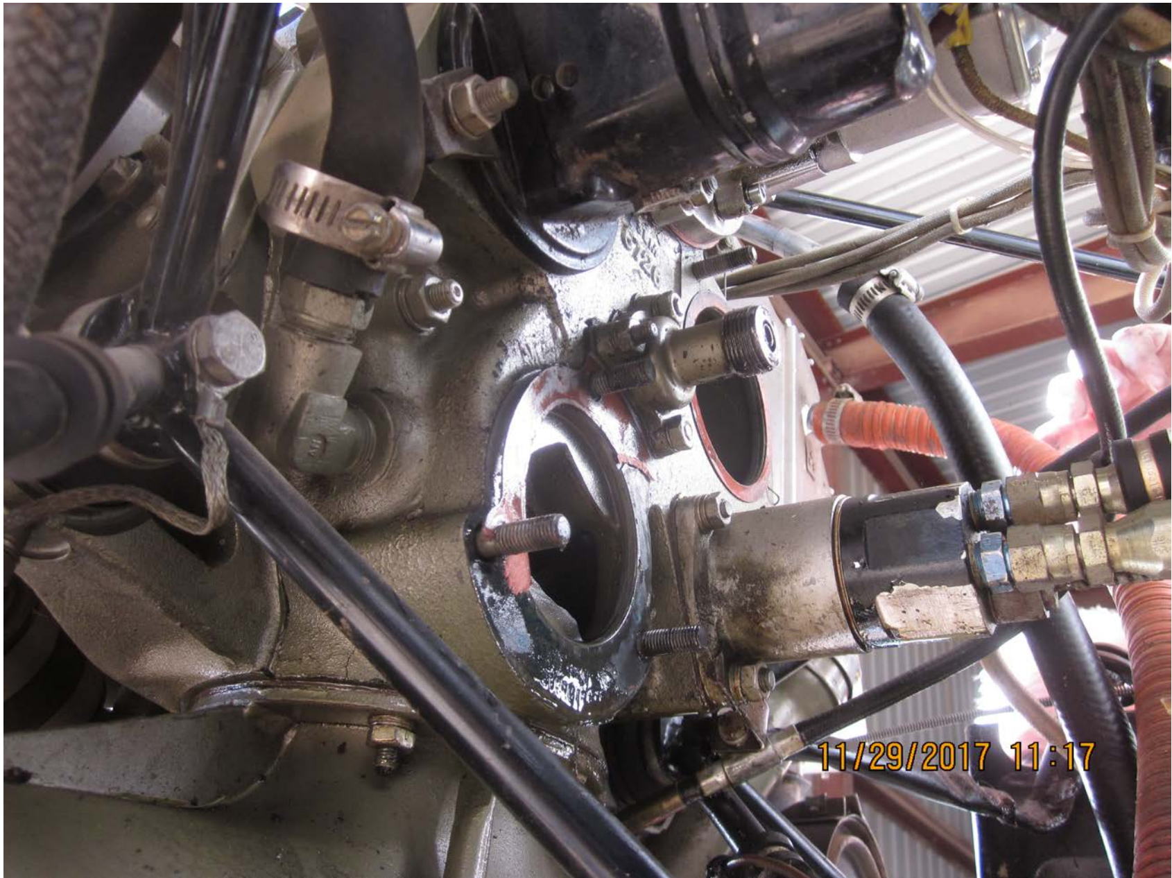
Photo 4 – Rear of engine
