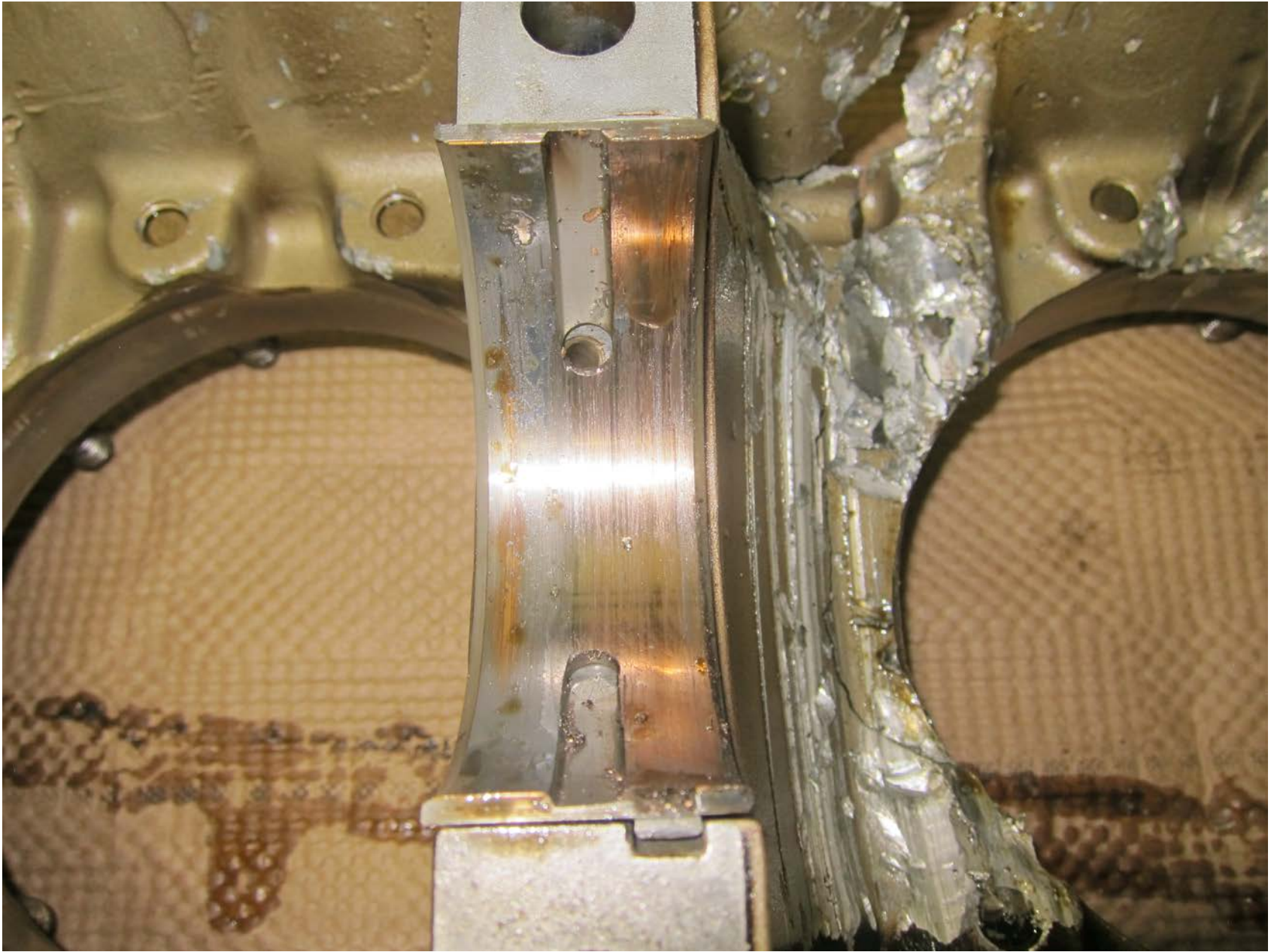
Photo 6 – View of No. 2 main bearing (CM Photo)
