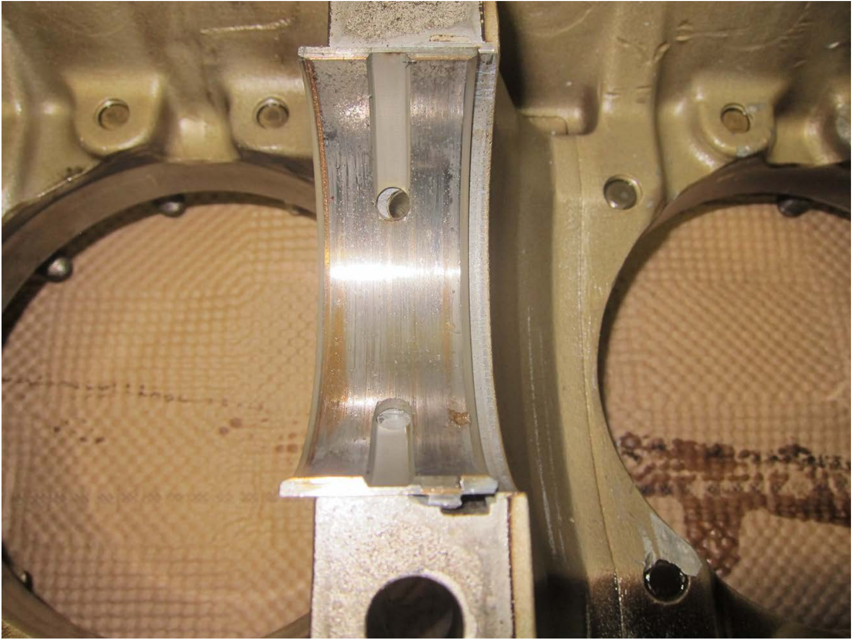
Photo 8 – View of No. 3 main bearing (CM Photo)
