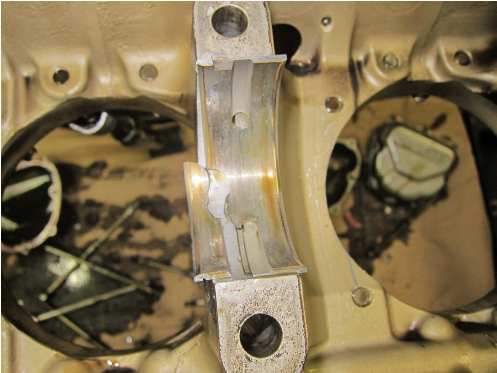
Photo 7 – View of No. 3 main bearing (CM Photo)
