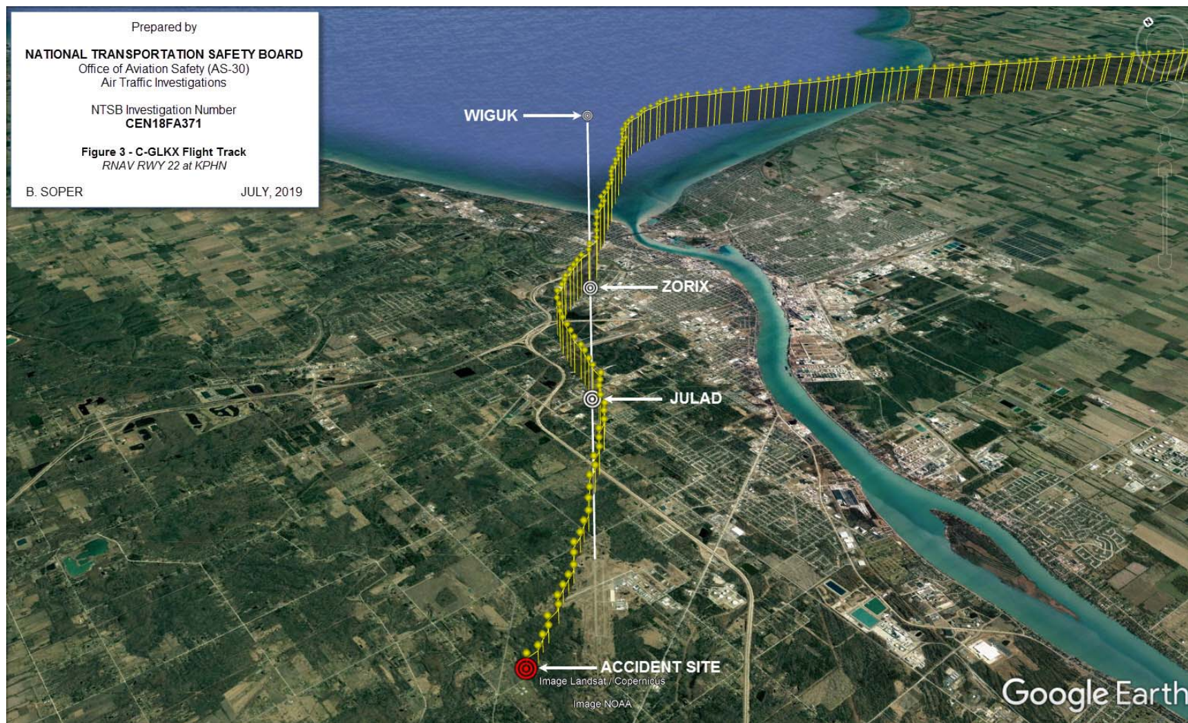
Figure 3 – Flight track of C-GLKX overlaid on satellite imagery with location of instrument approach fixes and RNAV runway 22 final approach course illustrated for reference.
