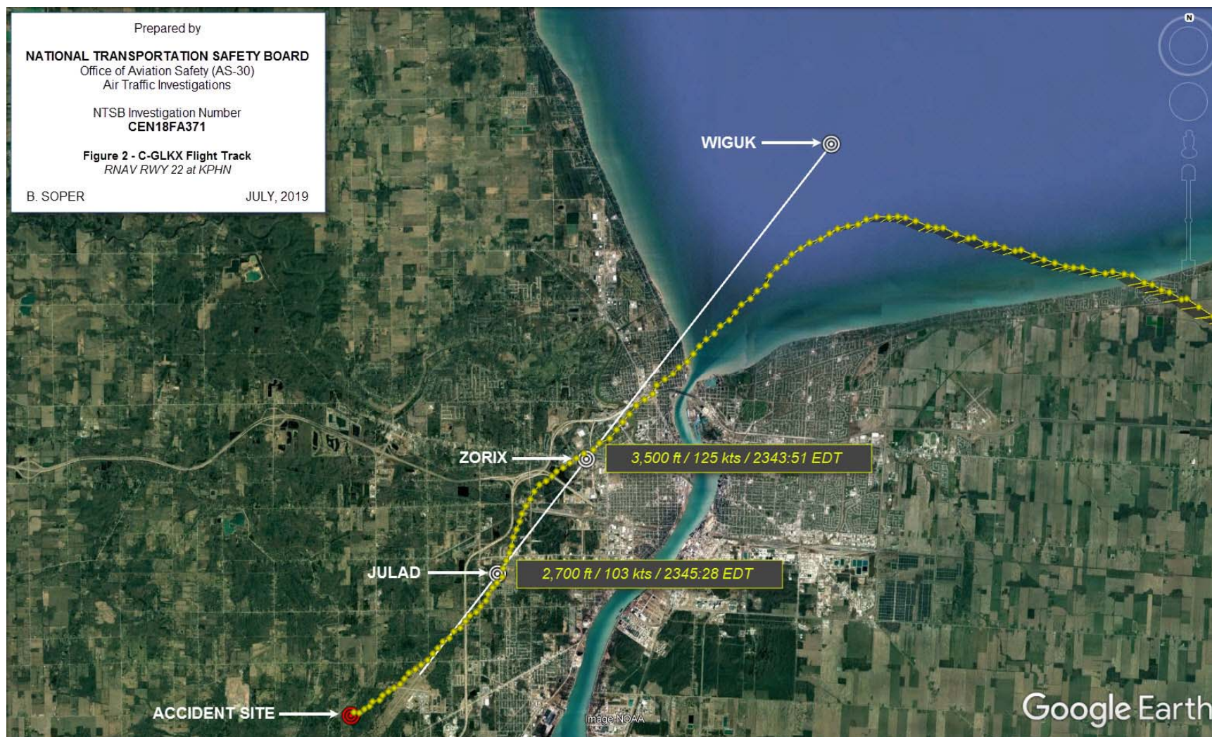
Figure 2 – Flight track of C-GLKX overlaid on satellite imagery with location of instrument approach fixes and RNAV runway 22 final approach course illustrated for reference.
