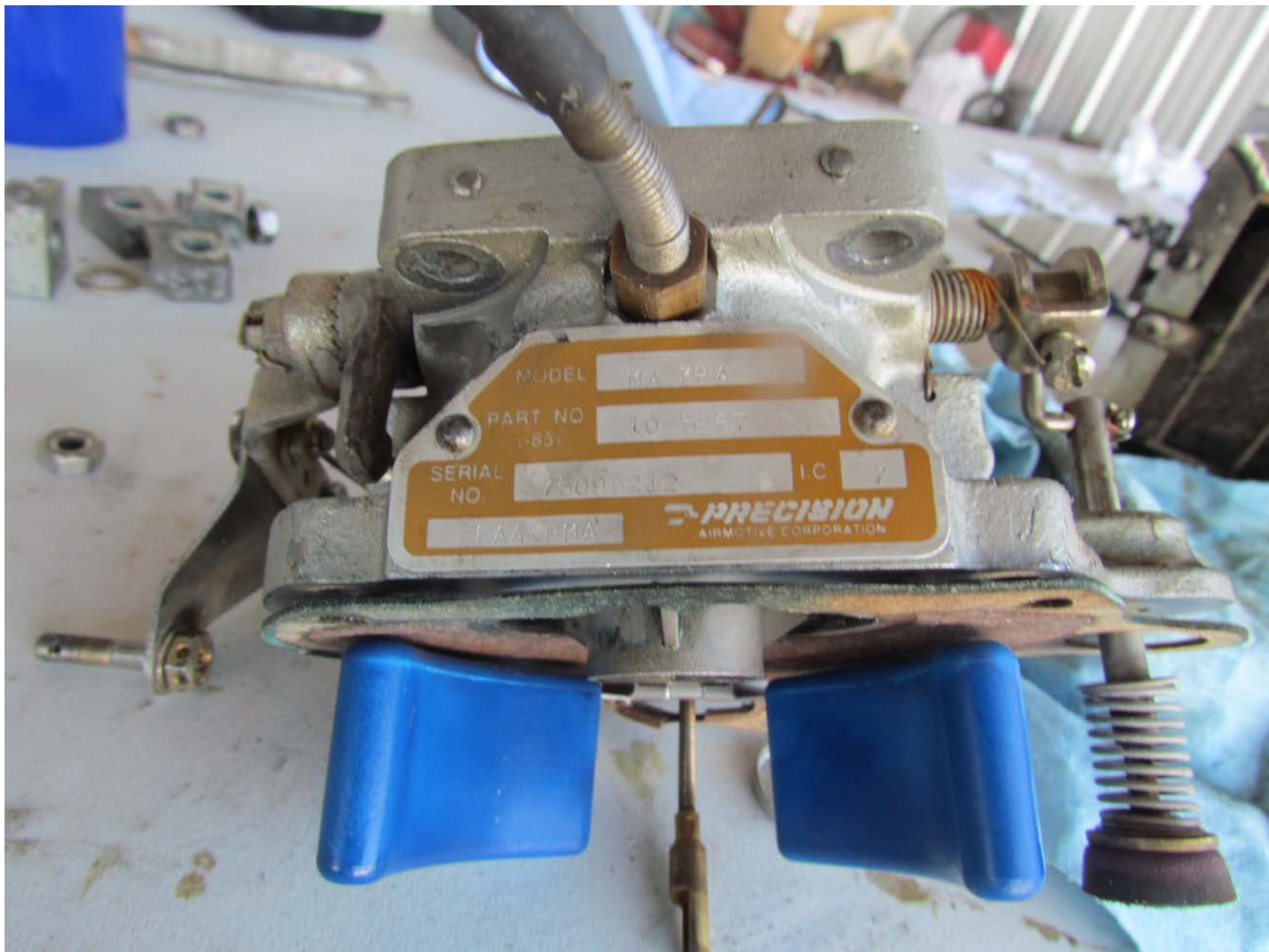
Photo 10 – View of the top portion of the carburetor (courtesy of Lycoming Engines).
