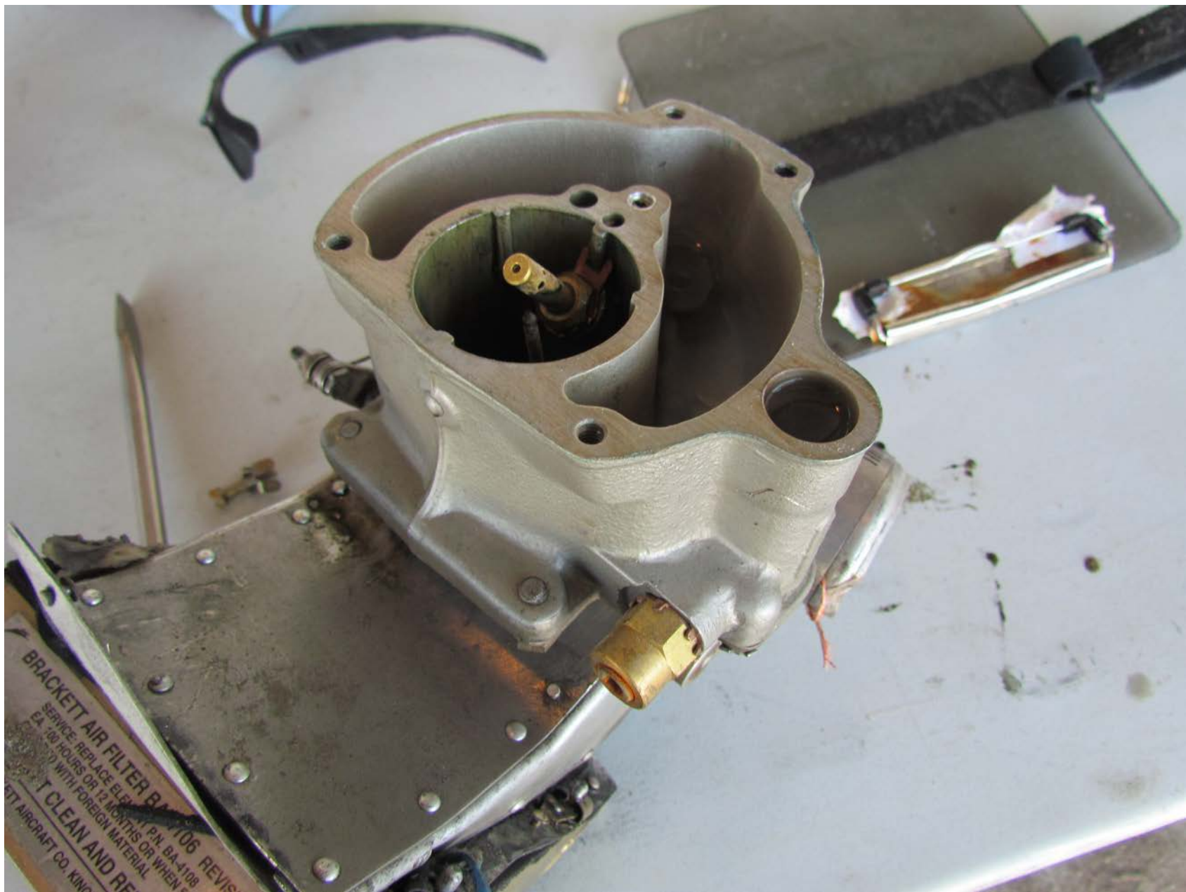
Photo 11 – View of the lower portion of the carburetor (courtesy of Lycoming Engines).
