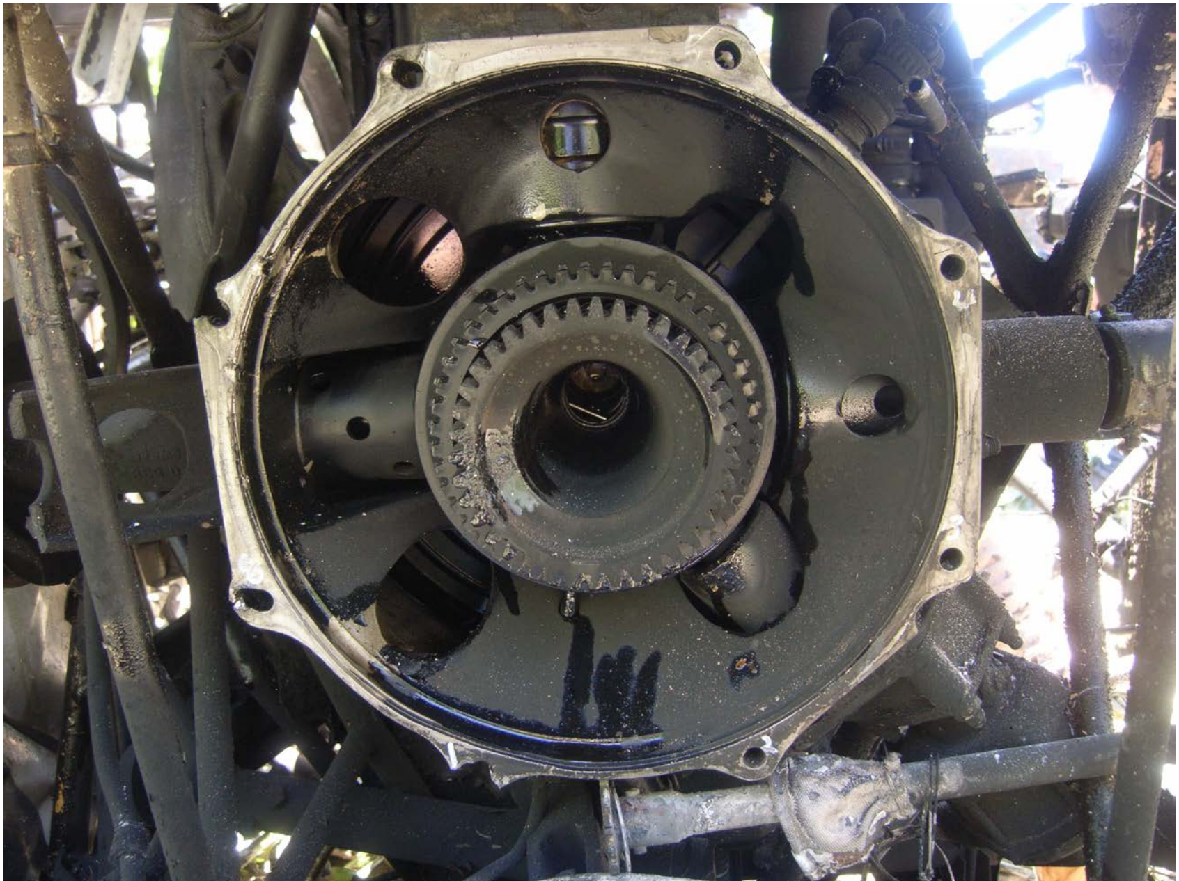
Photograph 8 - Lower Transmission
