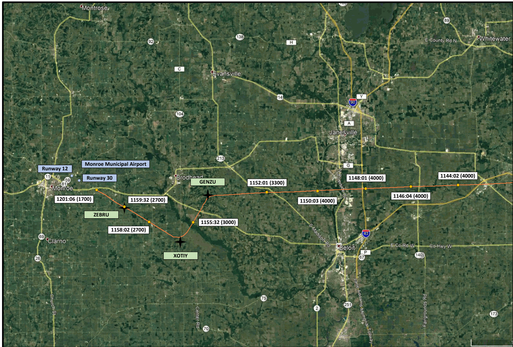
Figure 1 – Enroute and Approach Flight Segments
