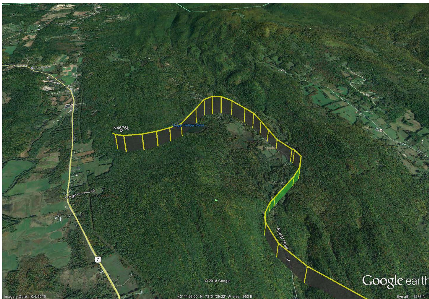
Figure 4 - GPS Plot of airplane within a valley before making a left turn and crossing one of the ridges forming the valley.
