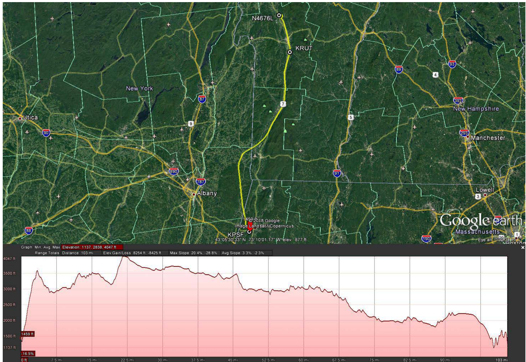
Figure 1 - Plotted GPS data of accident flight showing elevation profile.
