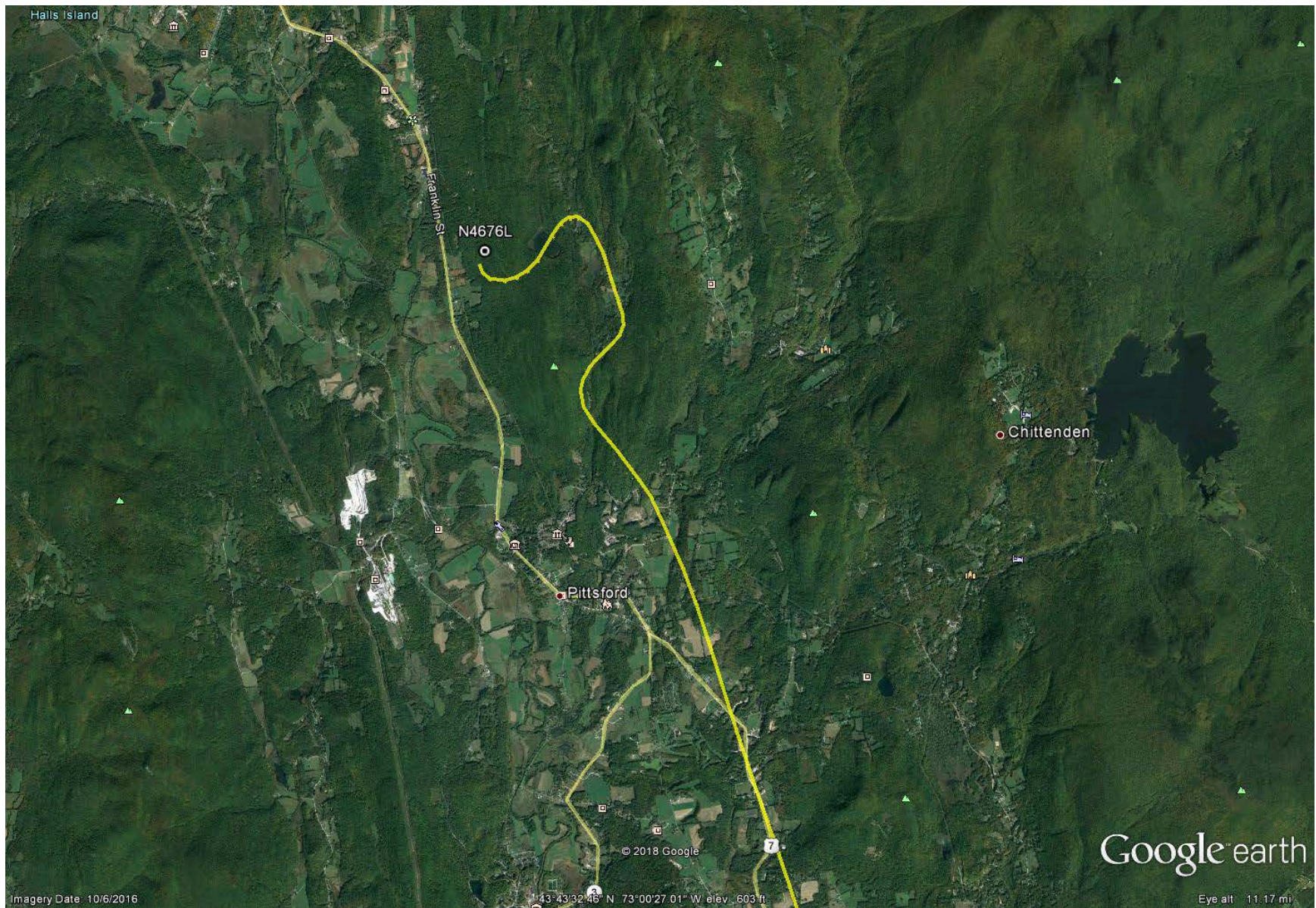
Figure 3 - GPS Plot showing the flight path diverging from the road where the road turns left.
