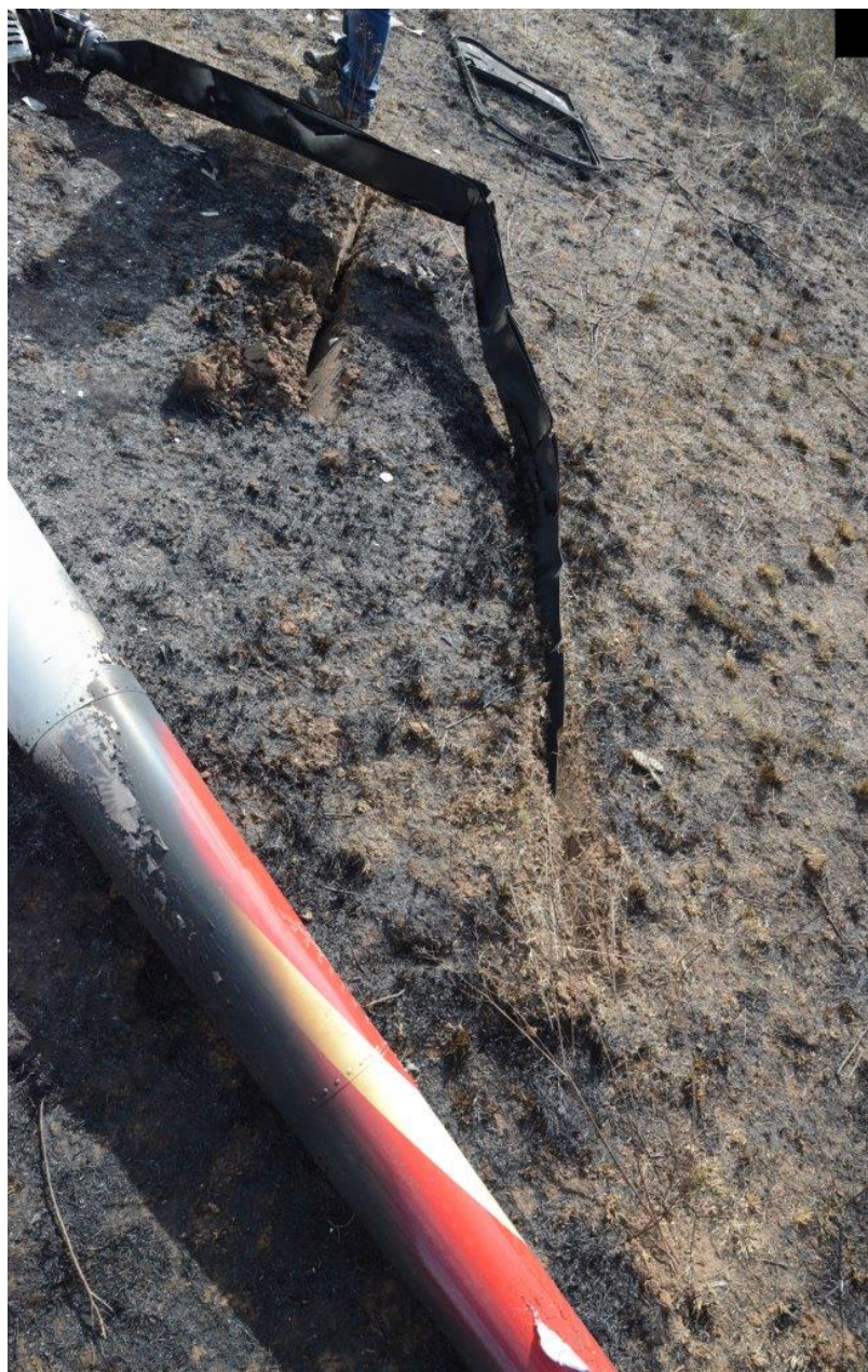
Photo 5 - View of the tailboom, main rotor blade, and ground scars.
