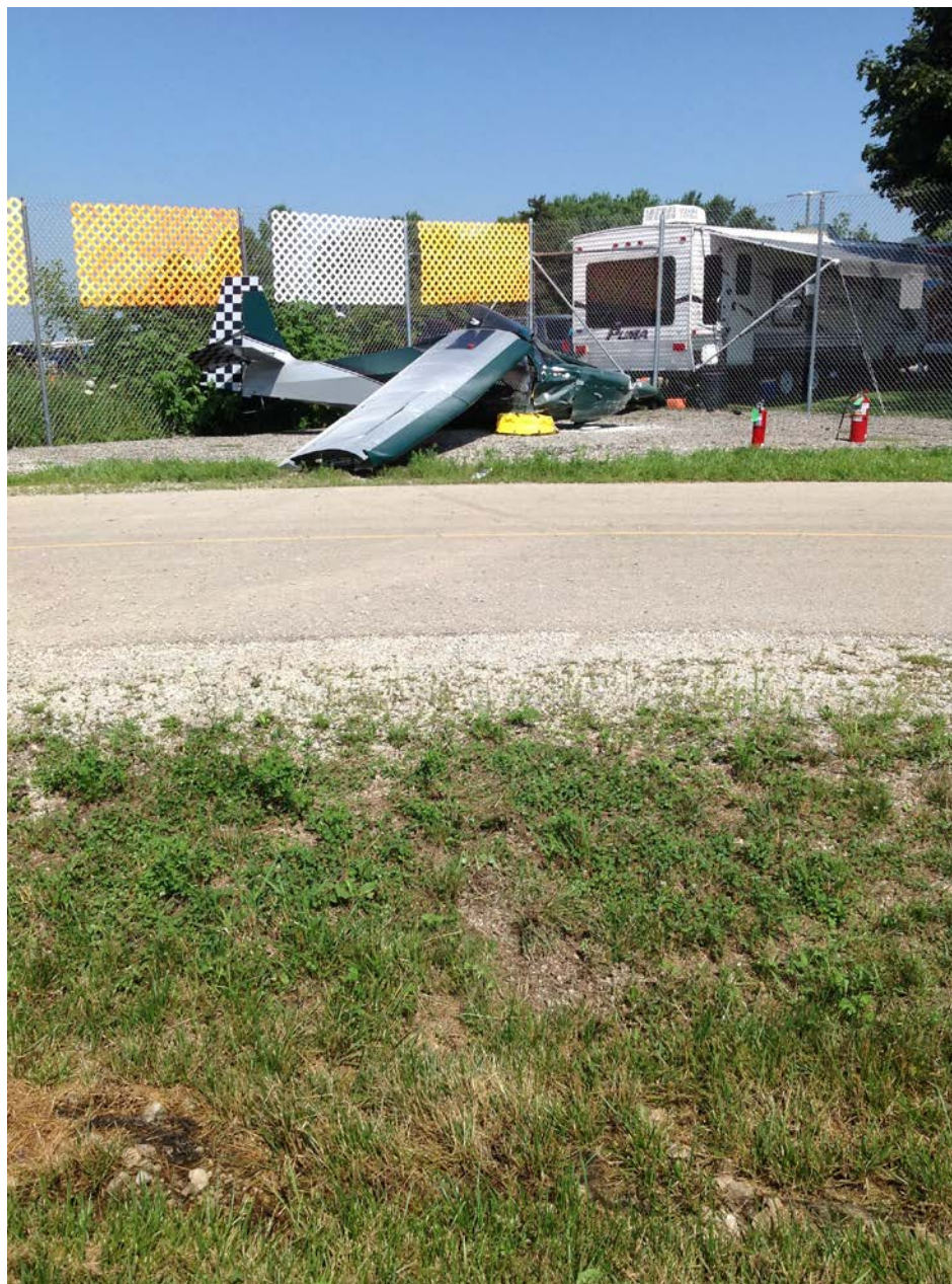
Photograph 01 - Initial impact point, ground scars, and right wing
