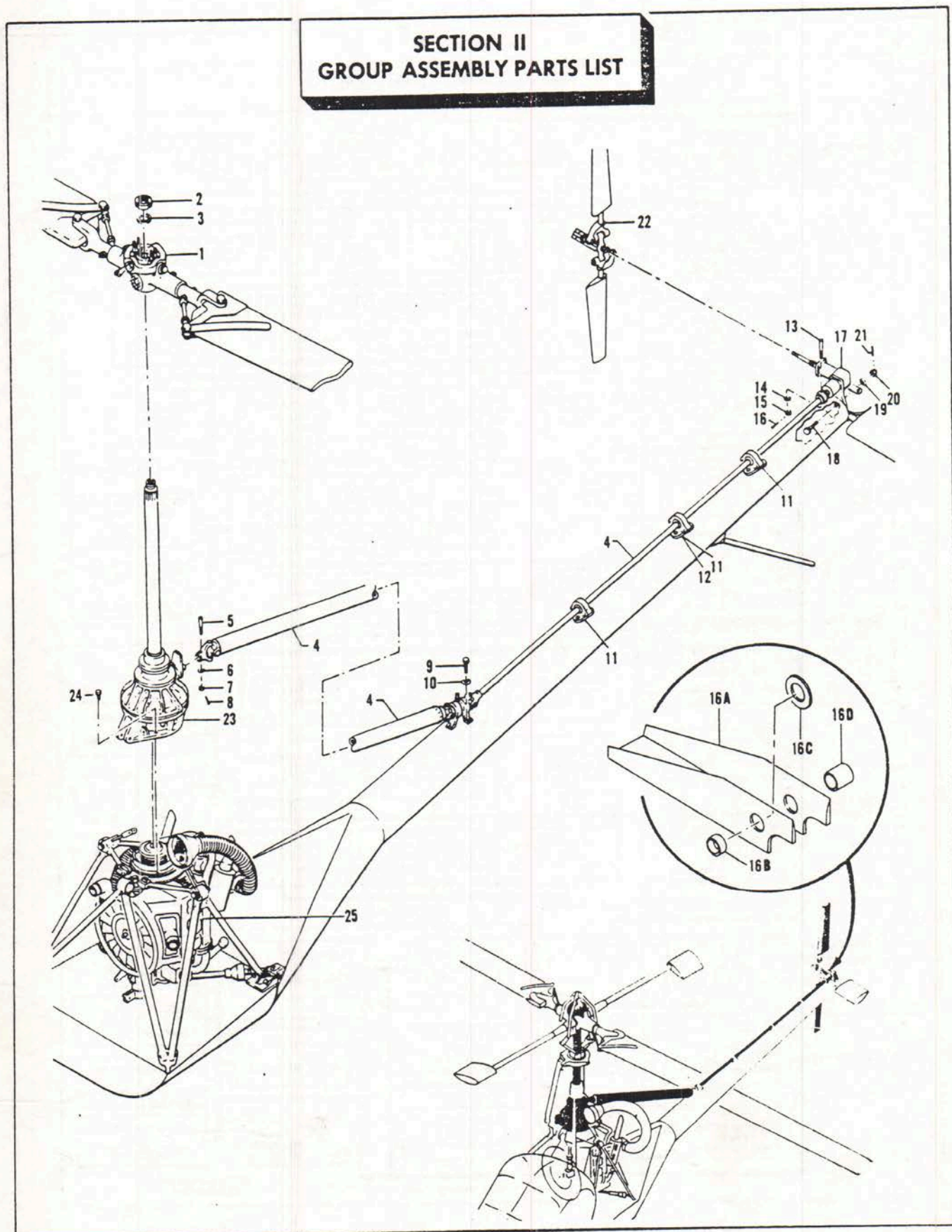
Figure 5. Rotors and Mechanical Drives Installation (UH-12A)
