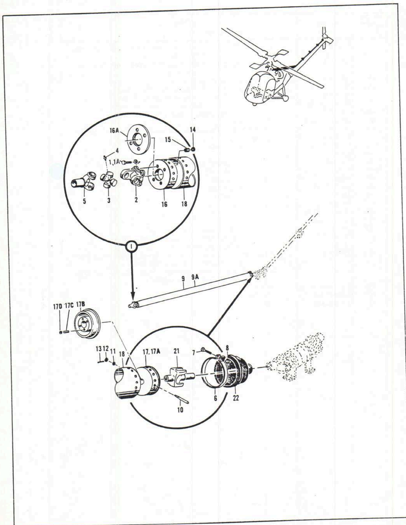
Figure 12. Tail Rotor Drive Assembly (UH-12A) (Sheet 1)
