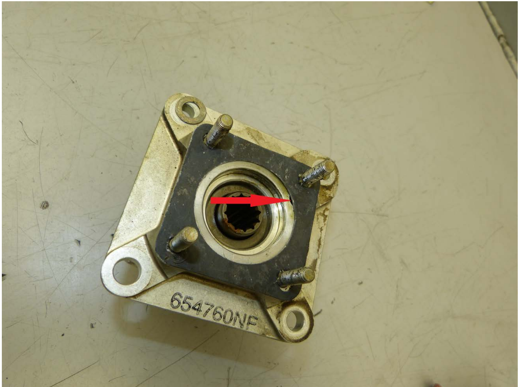
Photo 4 – Vacuum Pump Gasket as Discovered (Red Arrow Indicates Exposed Oil Orifice)
