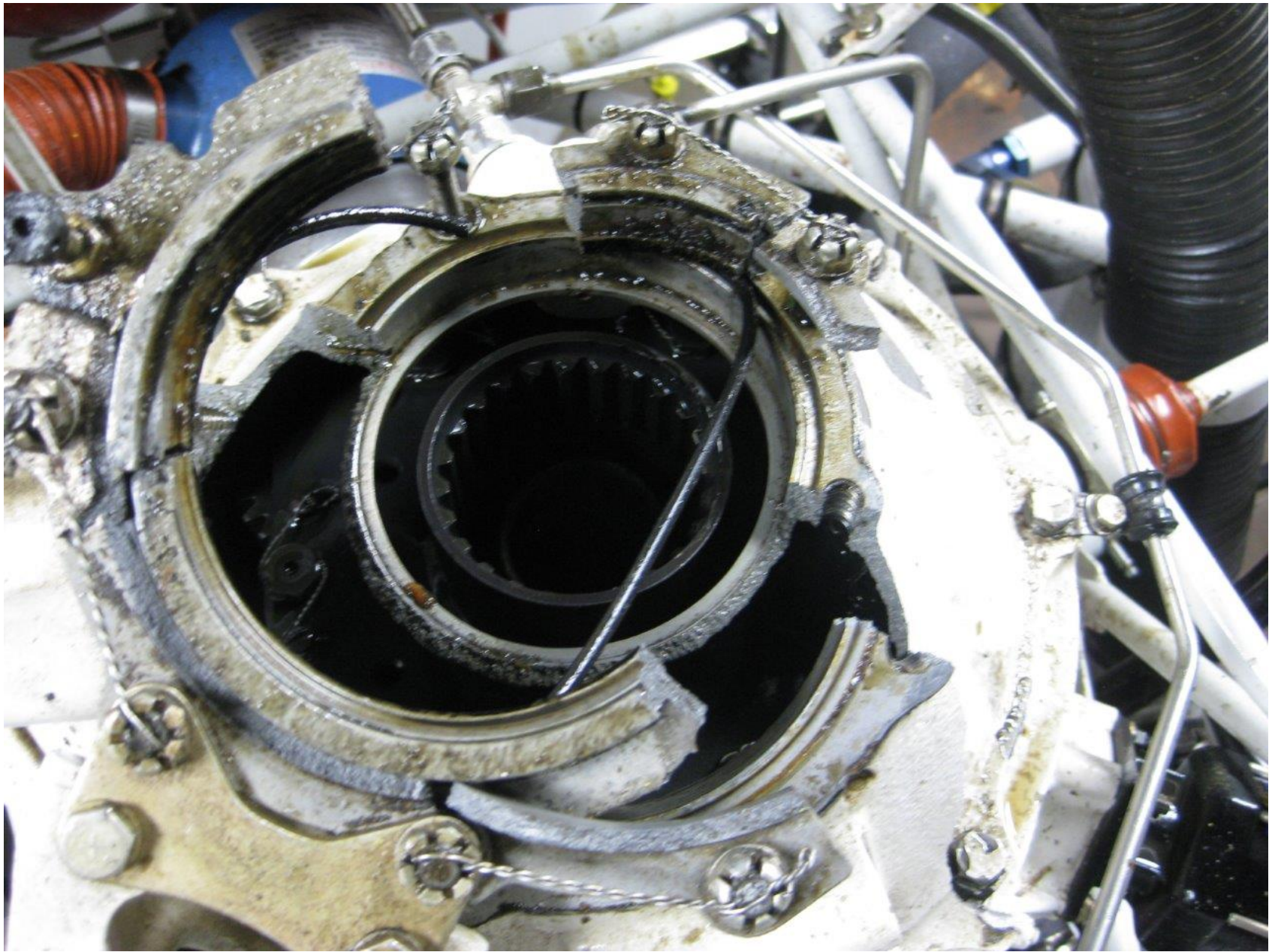
Photo 4 - View of the fractured transmission case.
