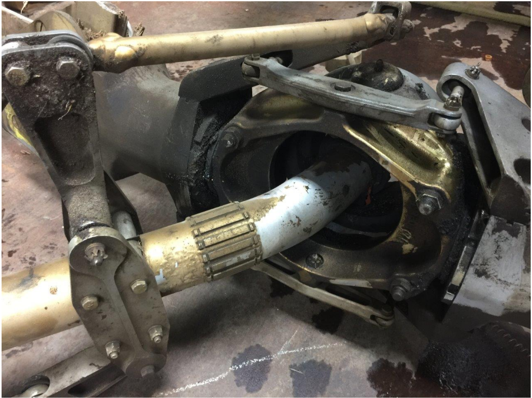
Photo 5 - Close-up view of the bent rotor mast,
