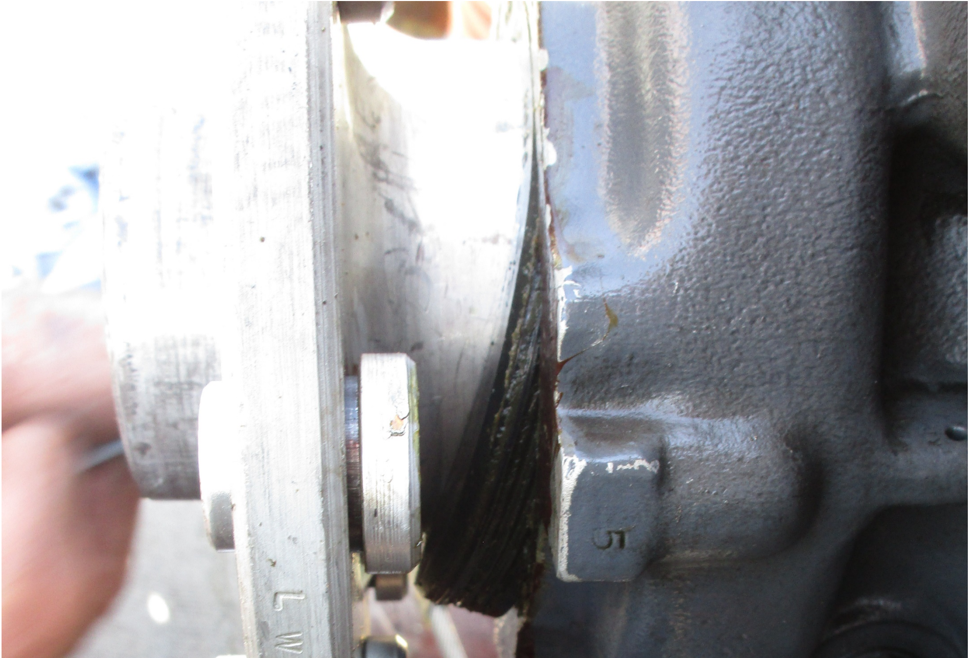
Photo 2 – Forward Main Seal (Crankshaft Seal)
