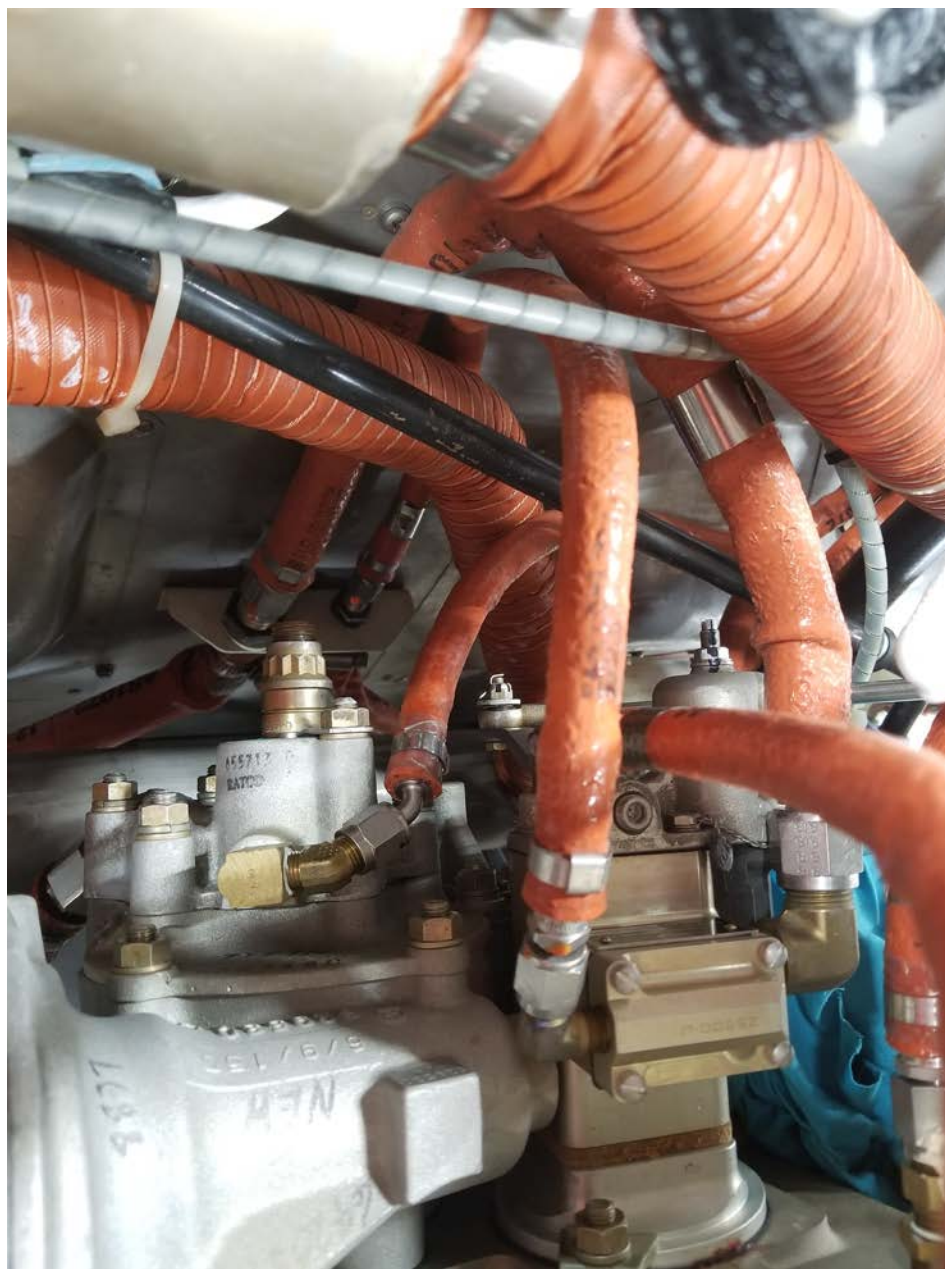
Photo 2 – View of hose routing on exemplar airplane at Mooney factory
