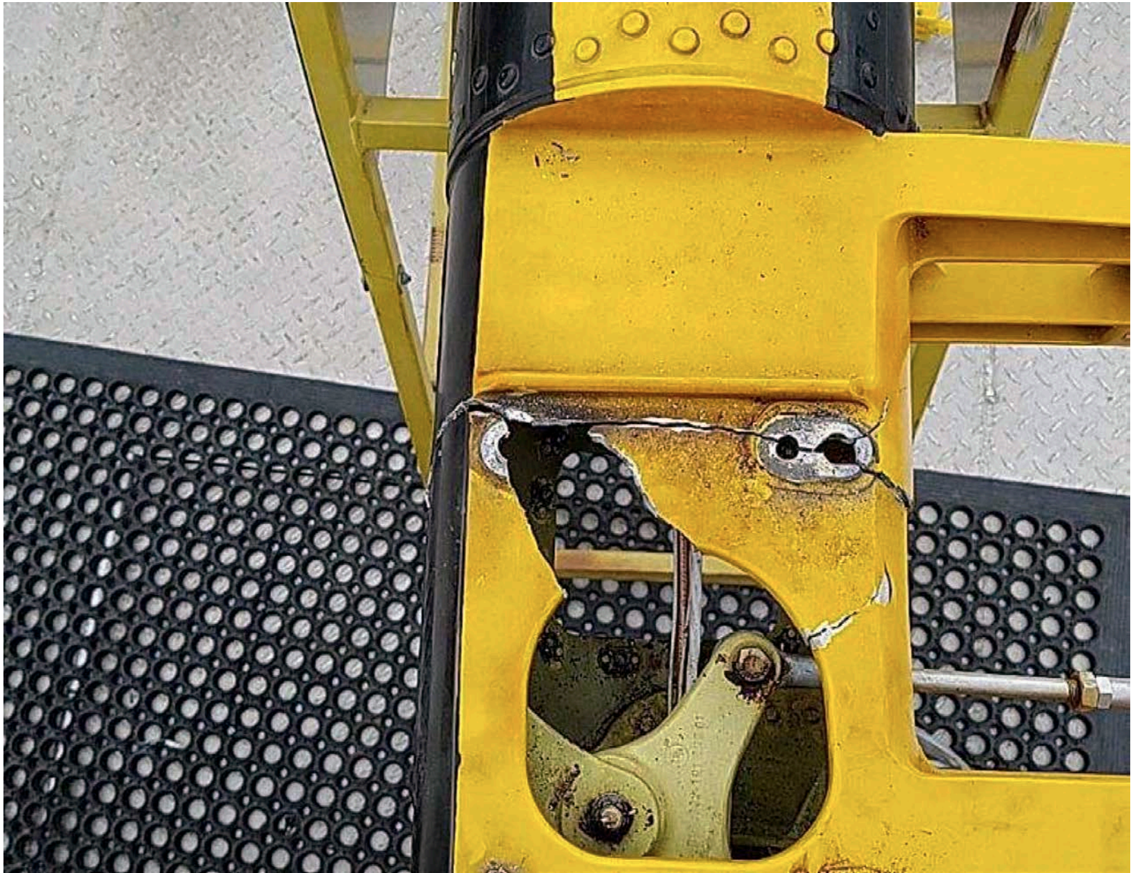
Photo 4 – Cracks in the tail boom support casting.
