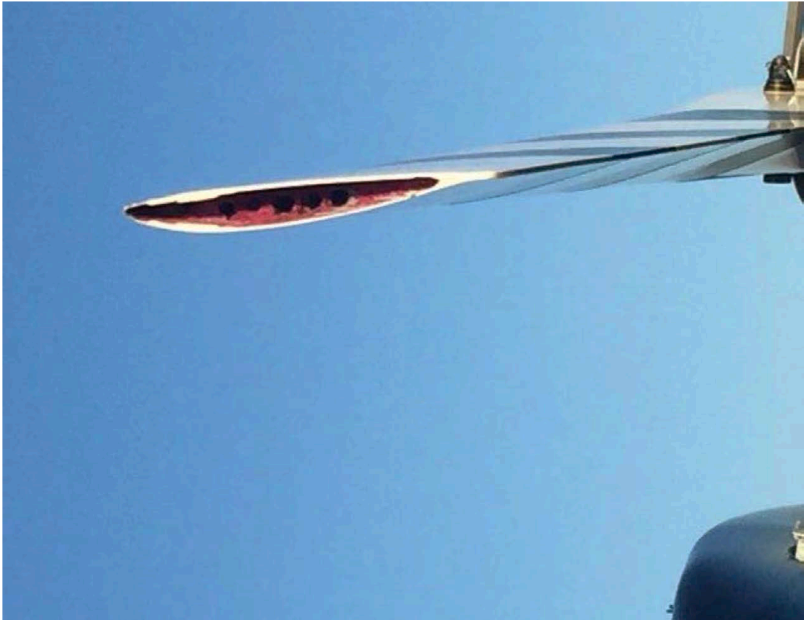
Photo 2 – Tail rotor blade with tip cap missing.
