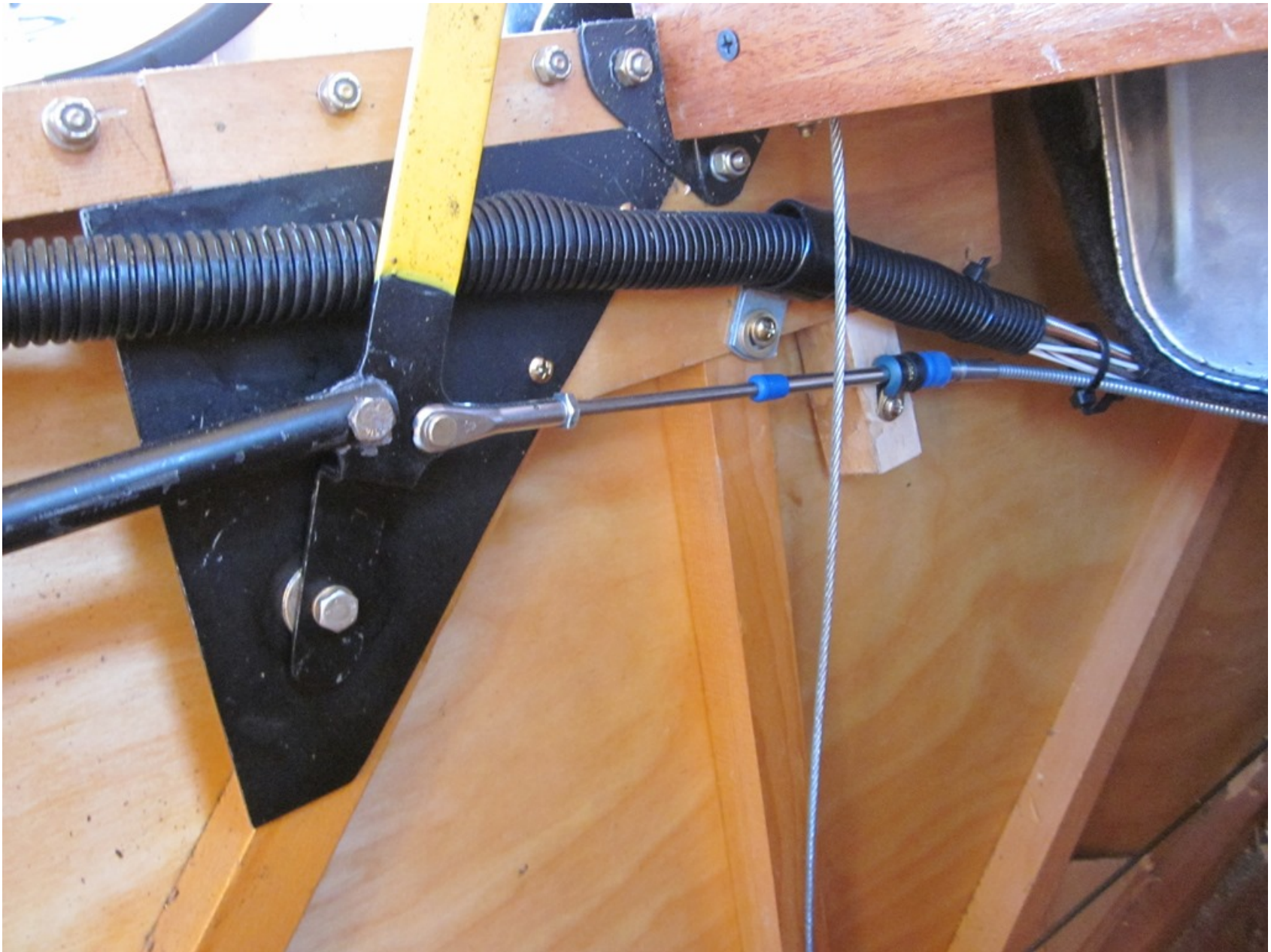
Photo 2 – Throttle Cable Mounting Block Separated
