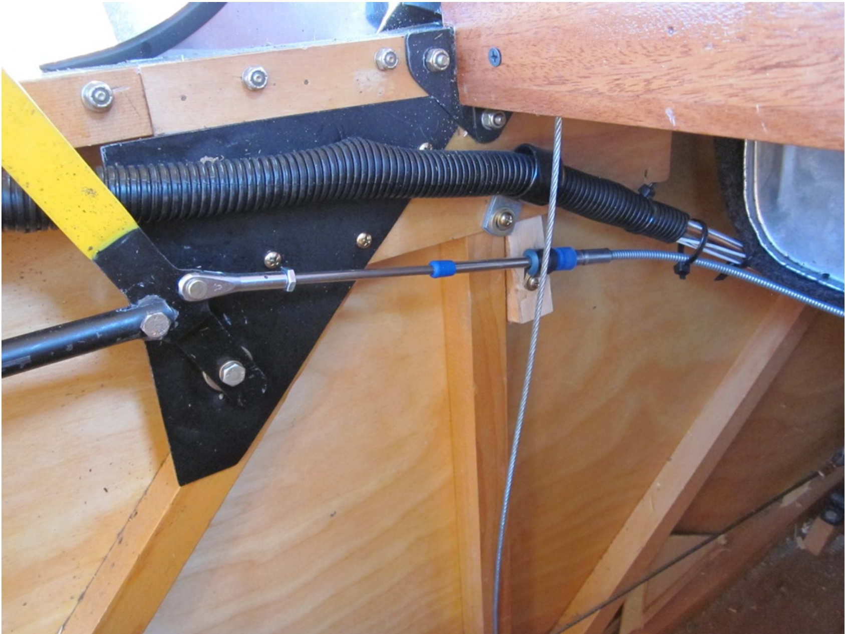
Photo 3 – Throttle Cable Mounting Block Re-Positioned in Original Location
