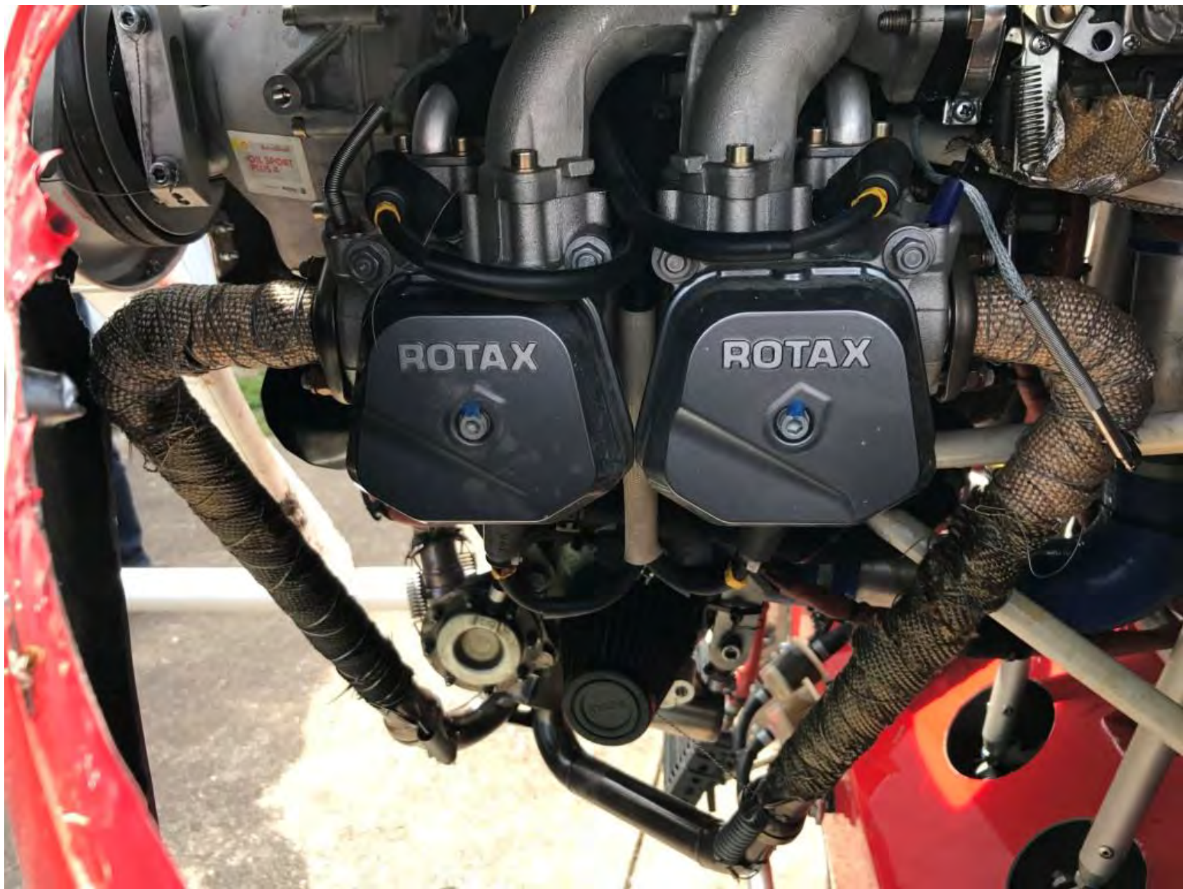
Photo 10 - View of the right side of the engine (looking aircraft forward)
