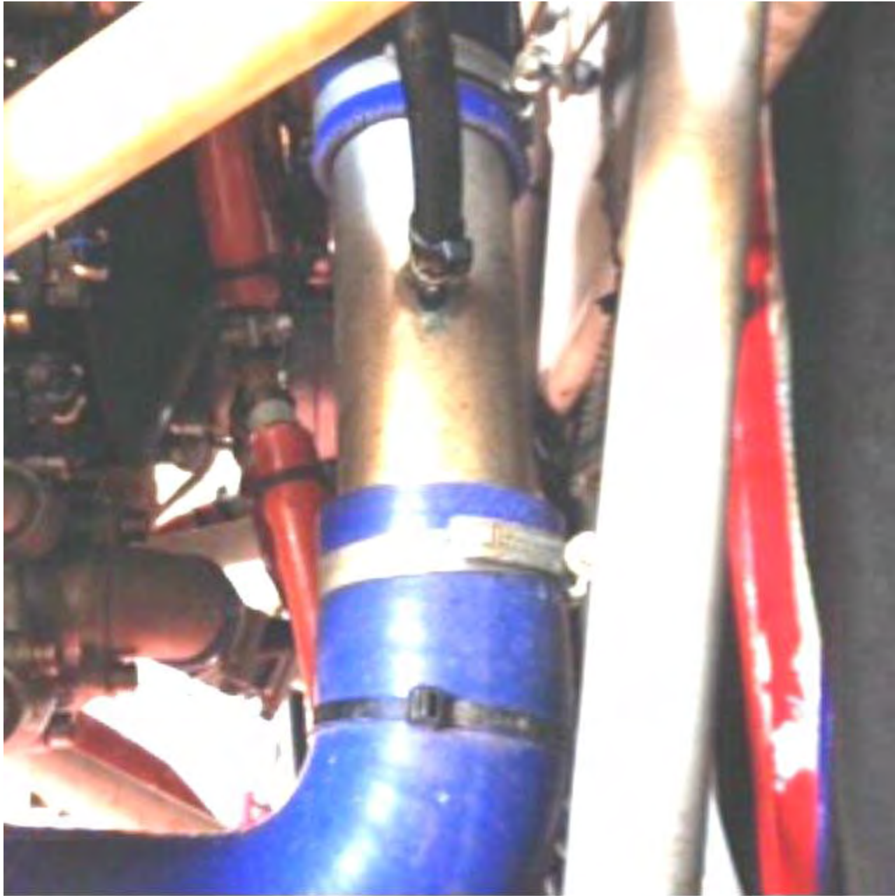
Photo 19 - Manifold pressure probe installation
