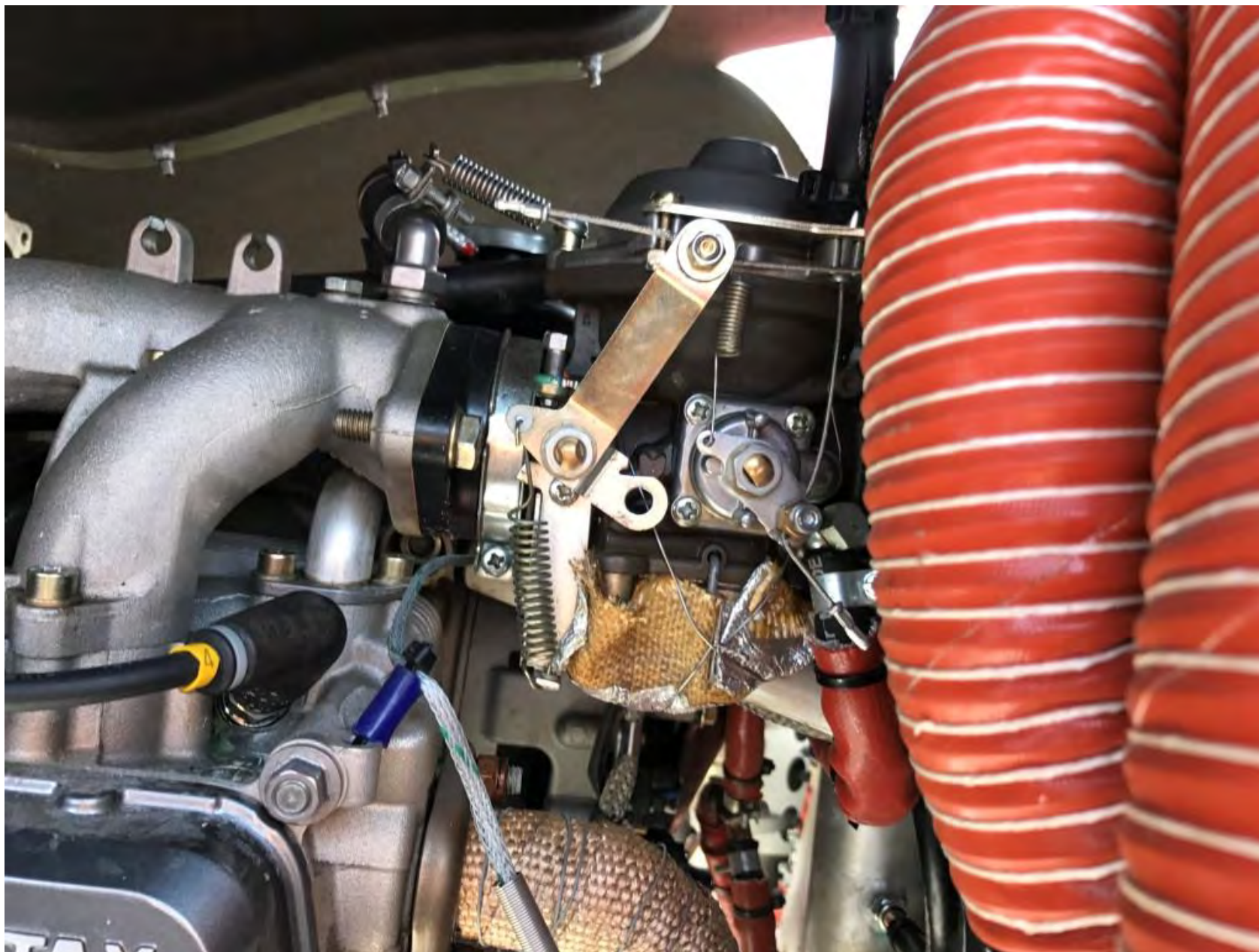
Photo 16 – View of right Bing carburetor
