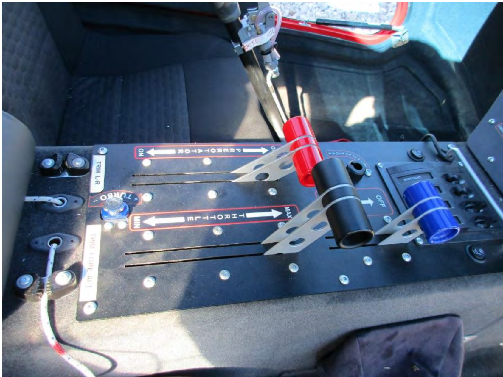
Photo 7 - View of the cockpit's power quadrant
