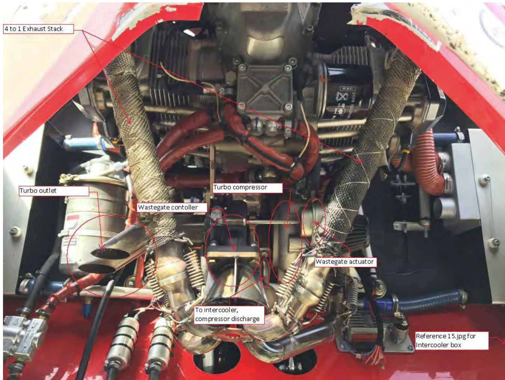
Photo 20 – View of engine with turbocharger parts identified
