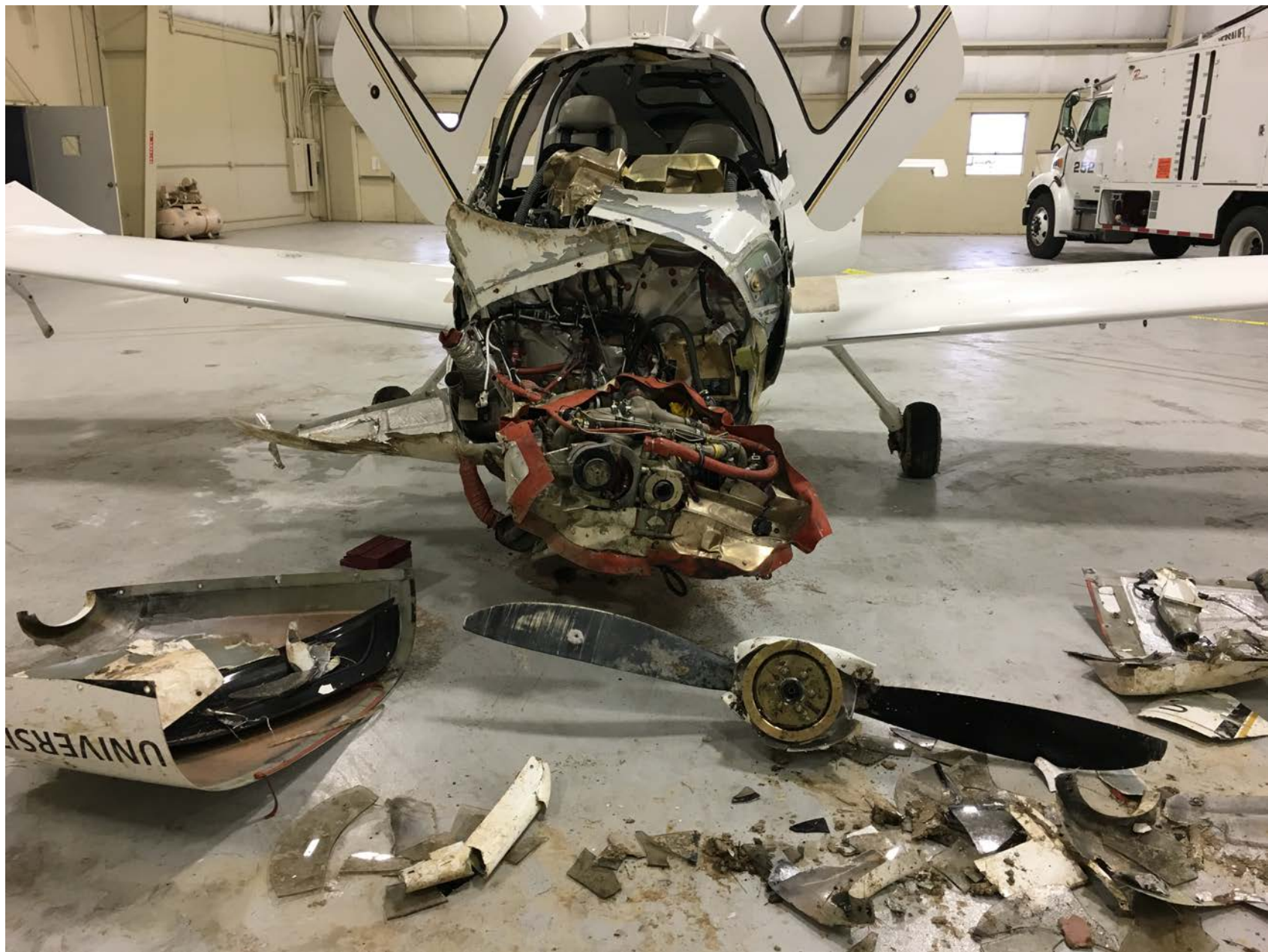
Photo 12 – View of engine, propeller and cowling
