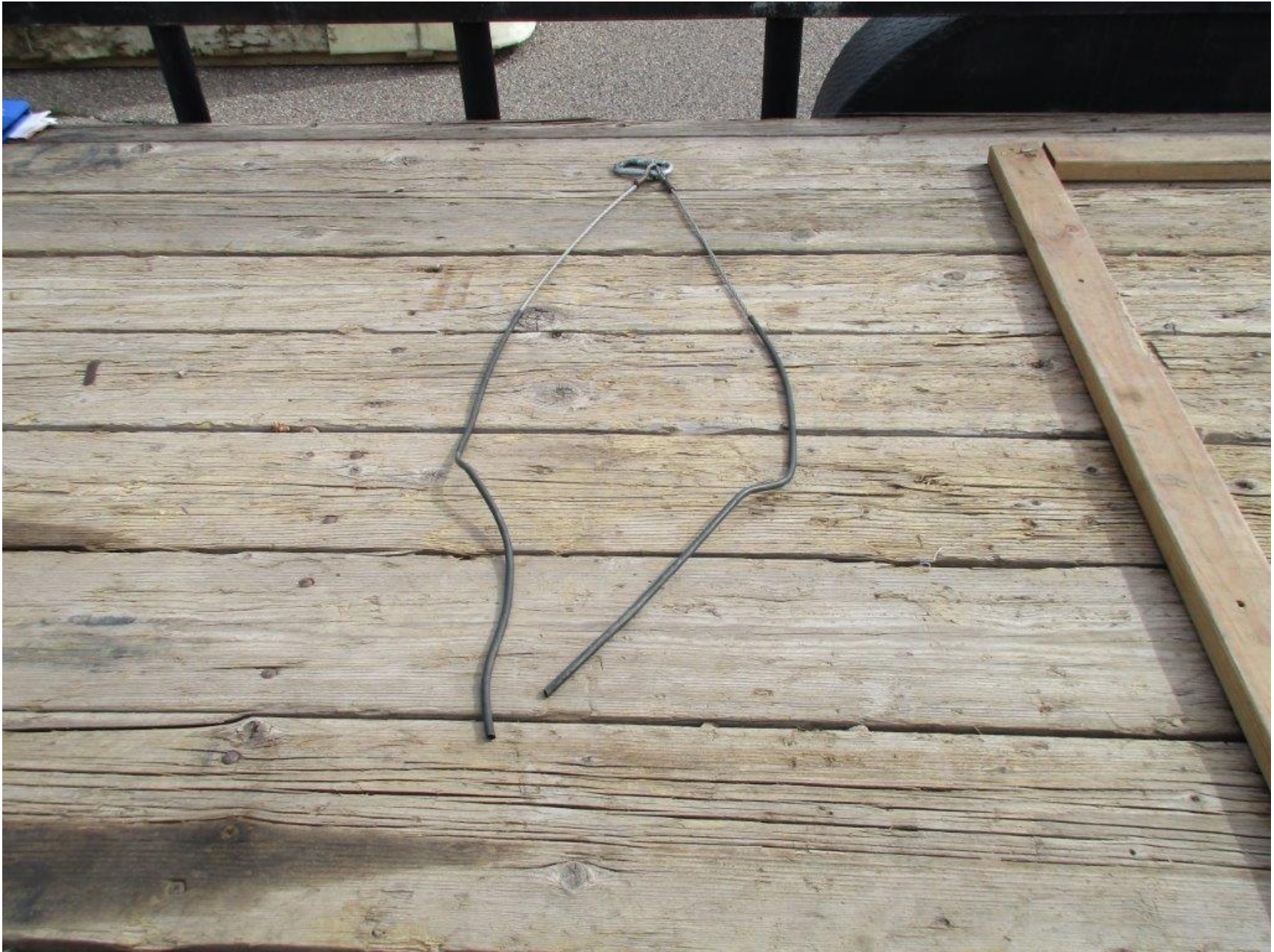
Photo 3 – Suspension Cables Damage
