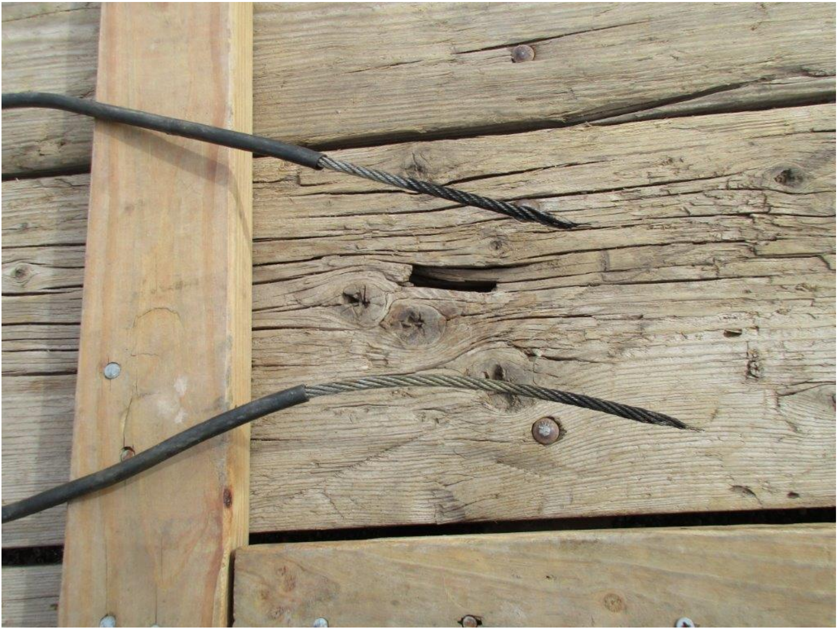
Photo 5 – Second Suspension Cables Damage, Detail
