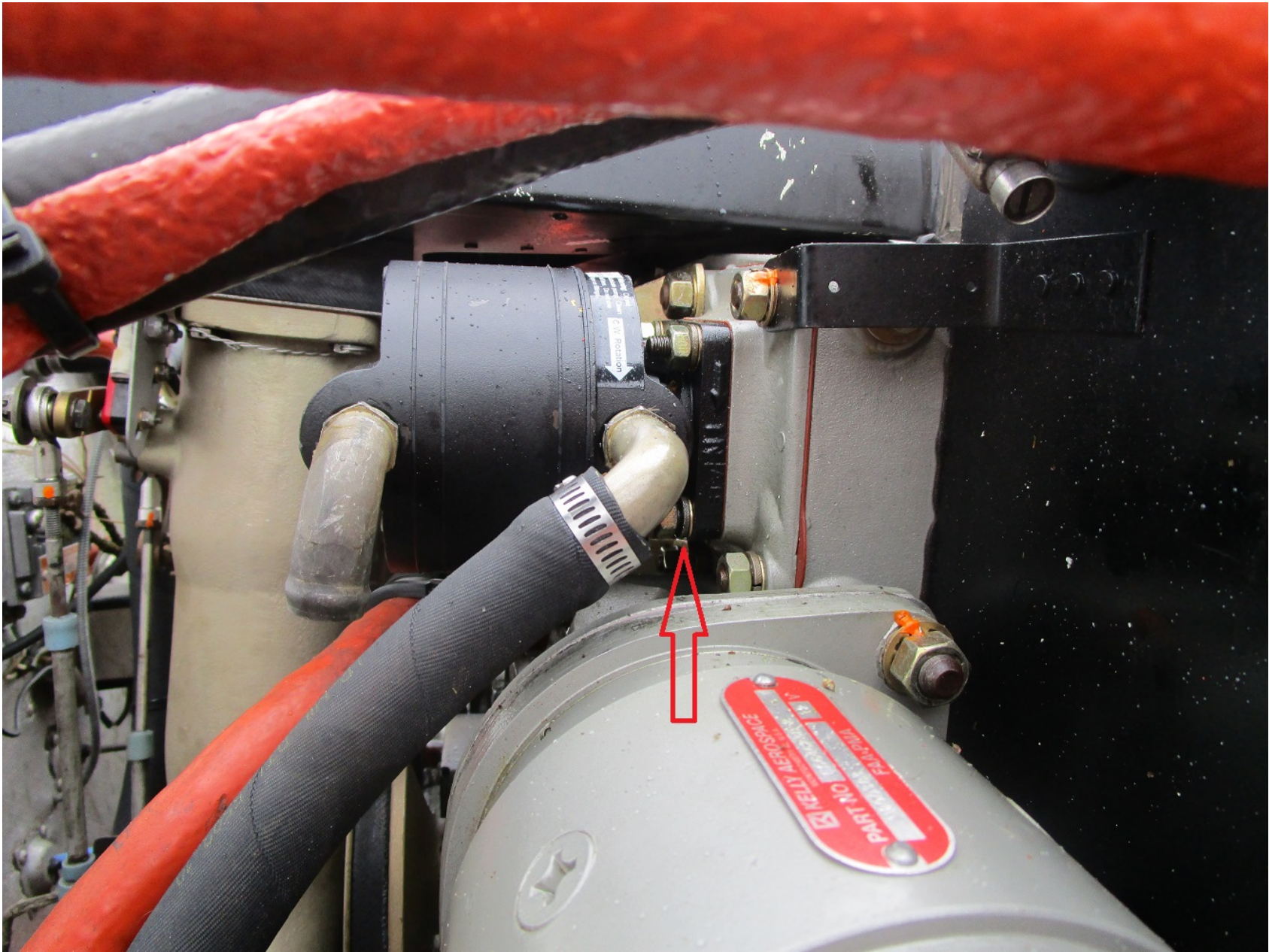
Photo 3 – Vacuum pump
