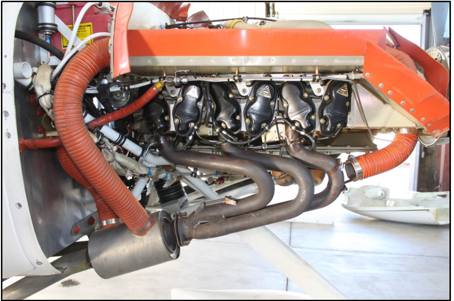
Photo 8 - Engine
