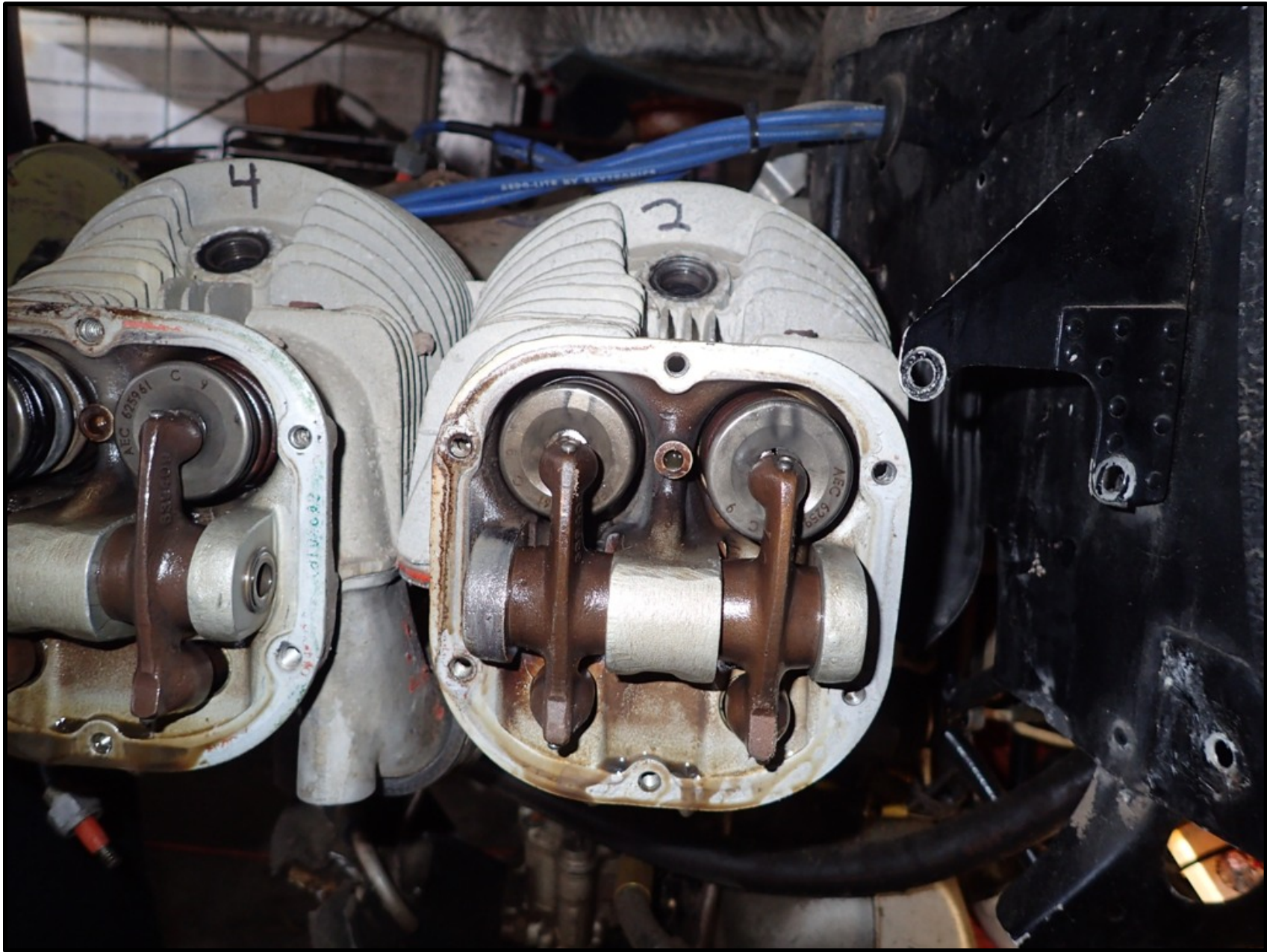
Photo 2 – No. 2 Cylinder
