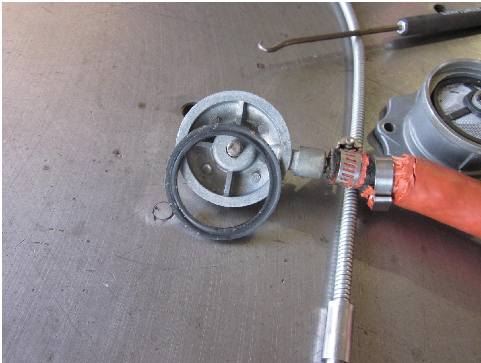
Photo 4 – Gasket (FAA Photo)
