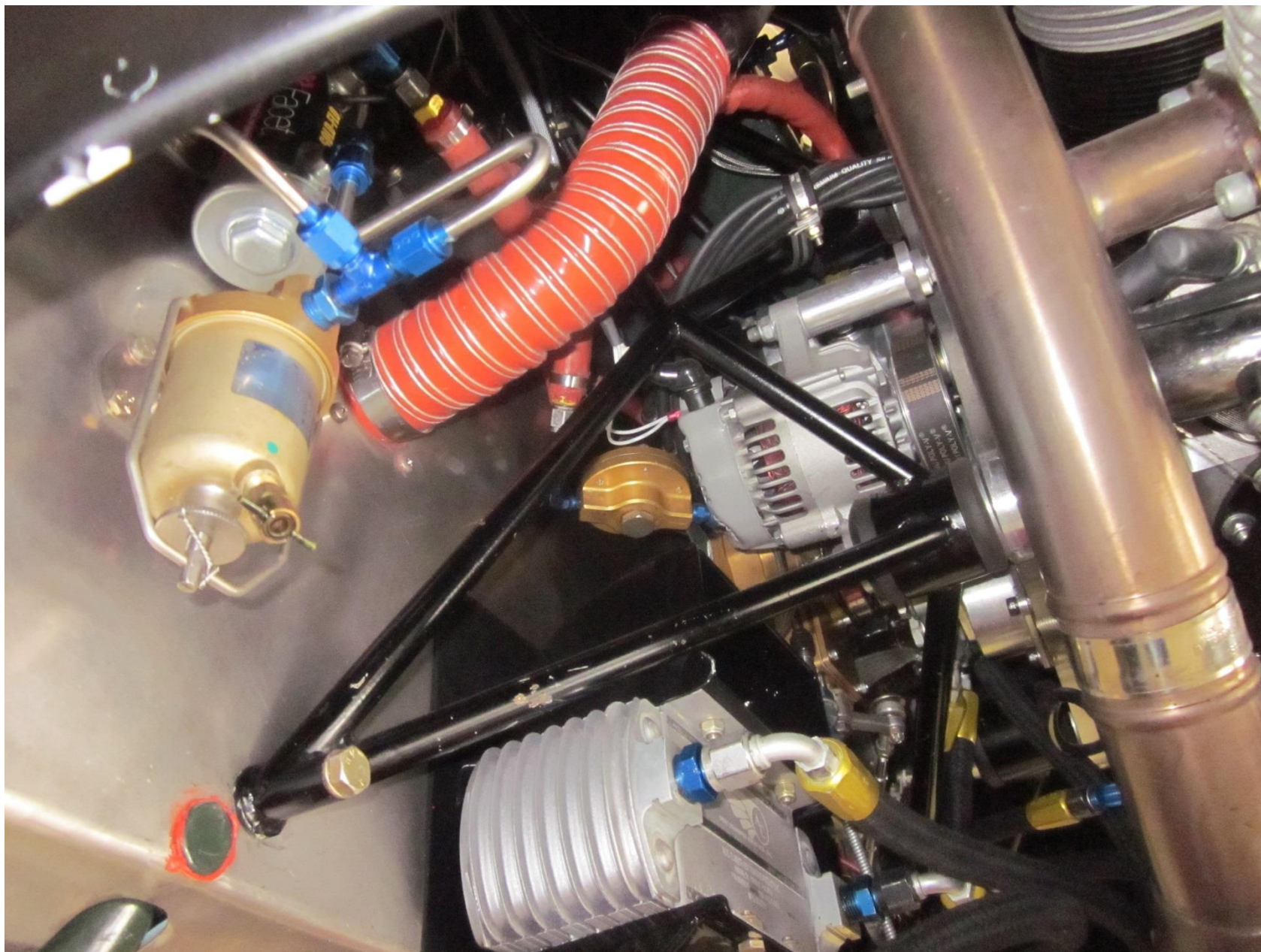
Photo 2 – Engine Accessories (FAA Photo)
