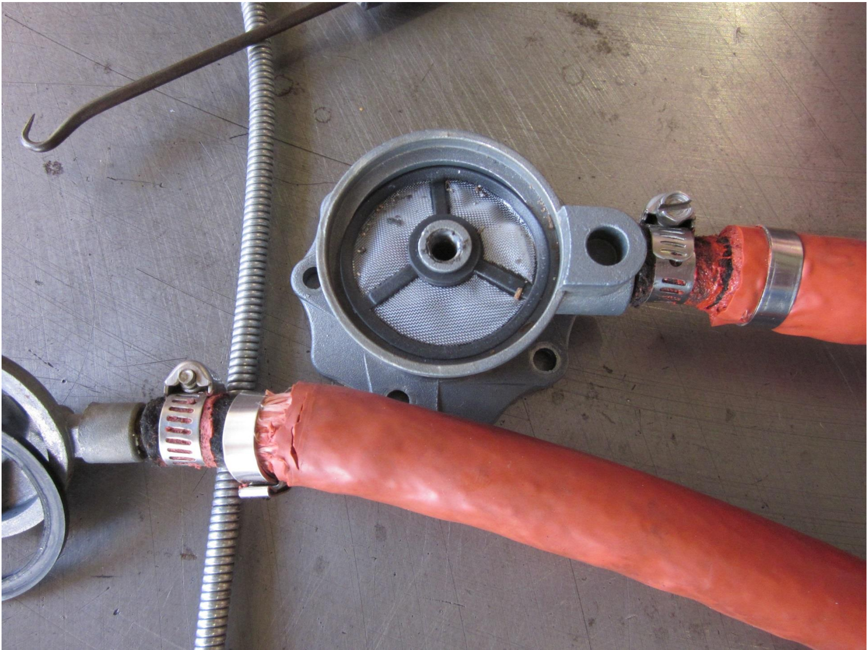
Photo 3 – Fuel Pump Screen (FAA Photo)
