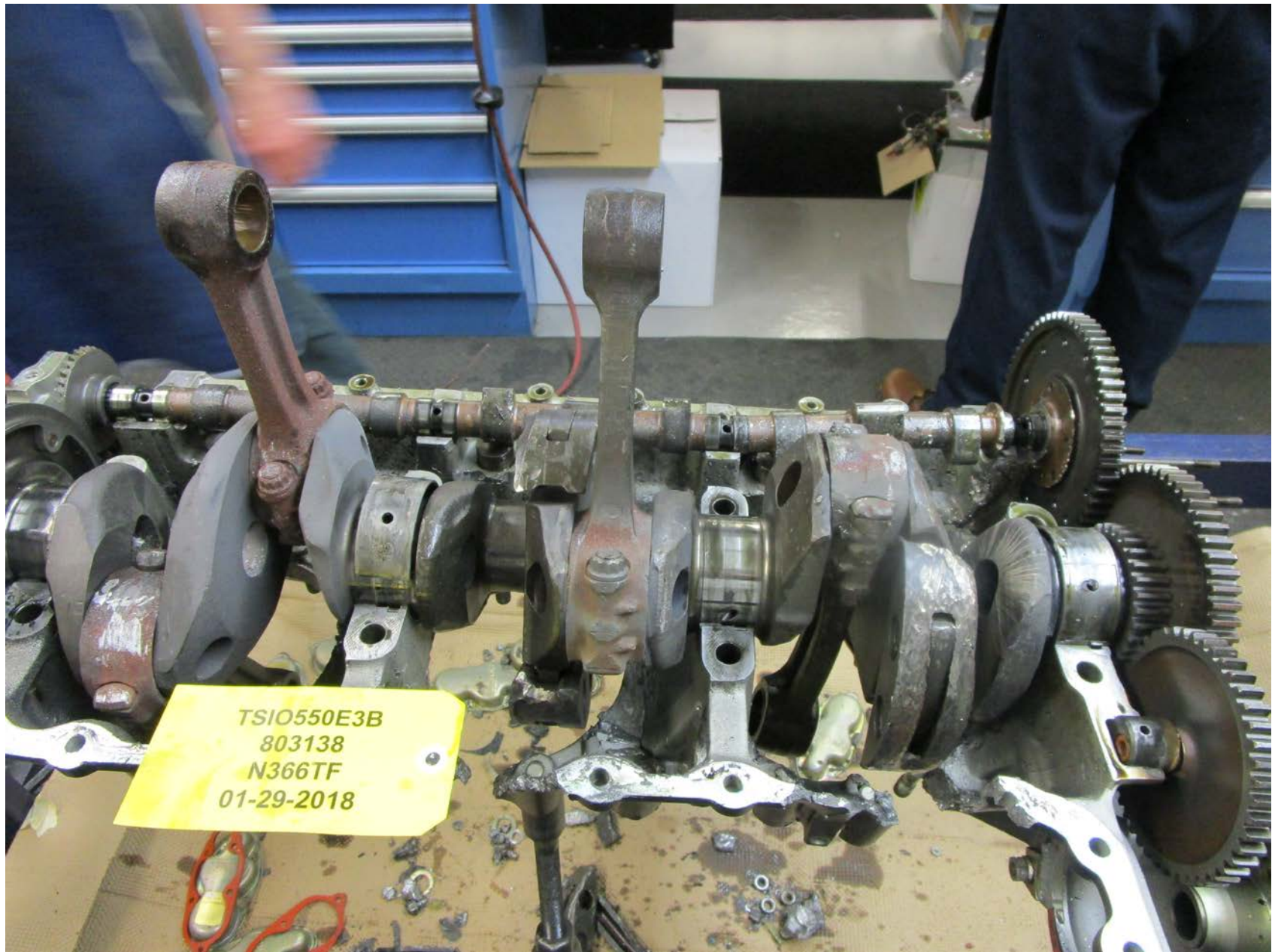
Photo 2 – Crankshaft with discolored connecting rods and bearings
