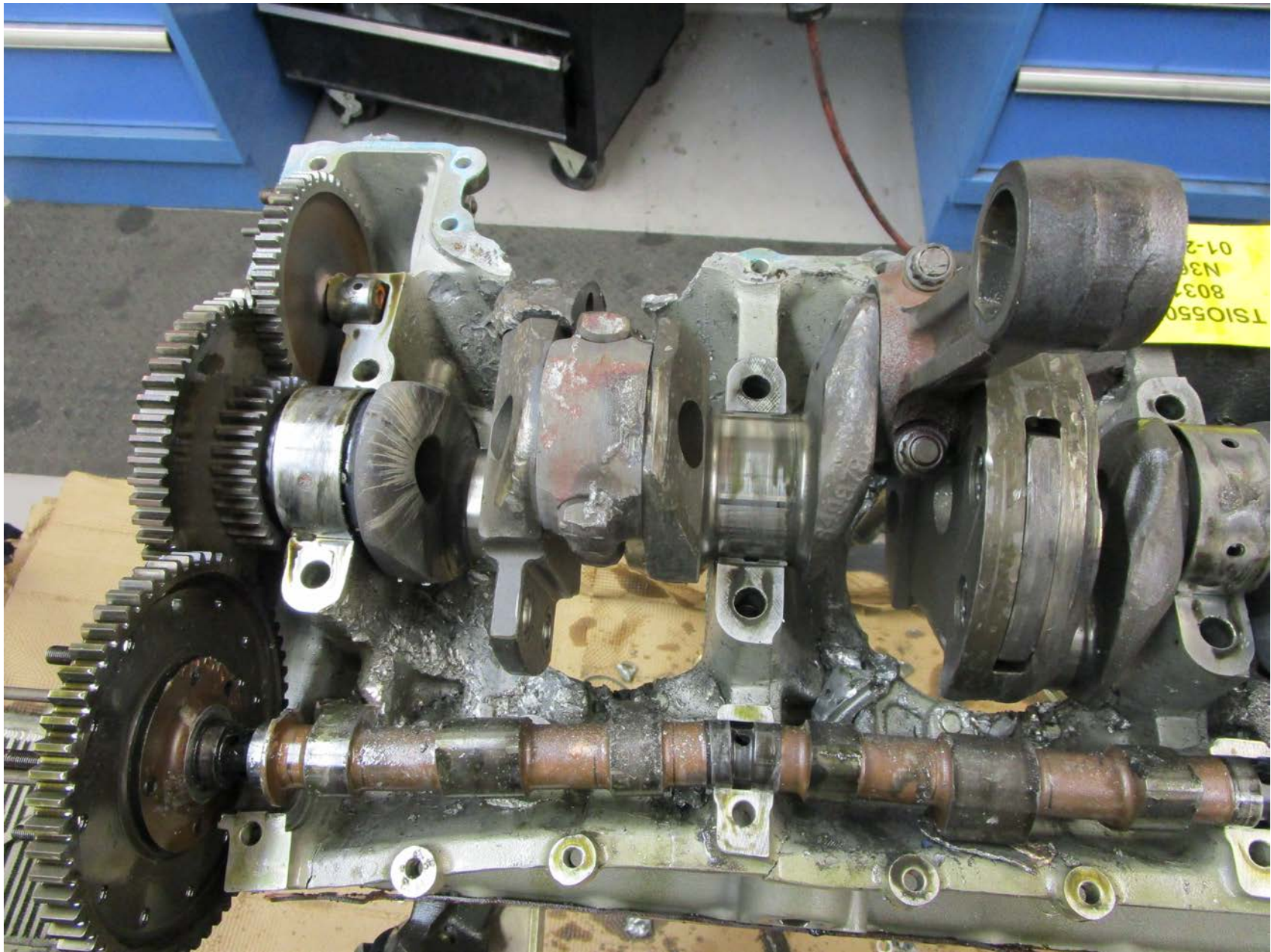
Photo 3 – Camshaft displaced from crankshaft
