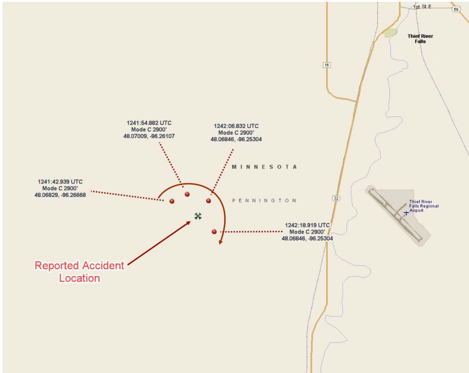
Radar Data Image 1 – Top View + Airport
