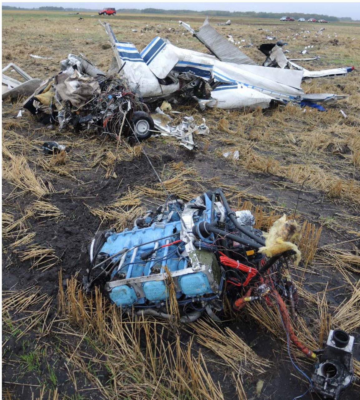
Photo 4 – Main Wreckage and Engine
