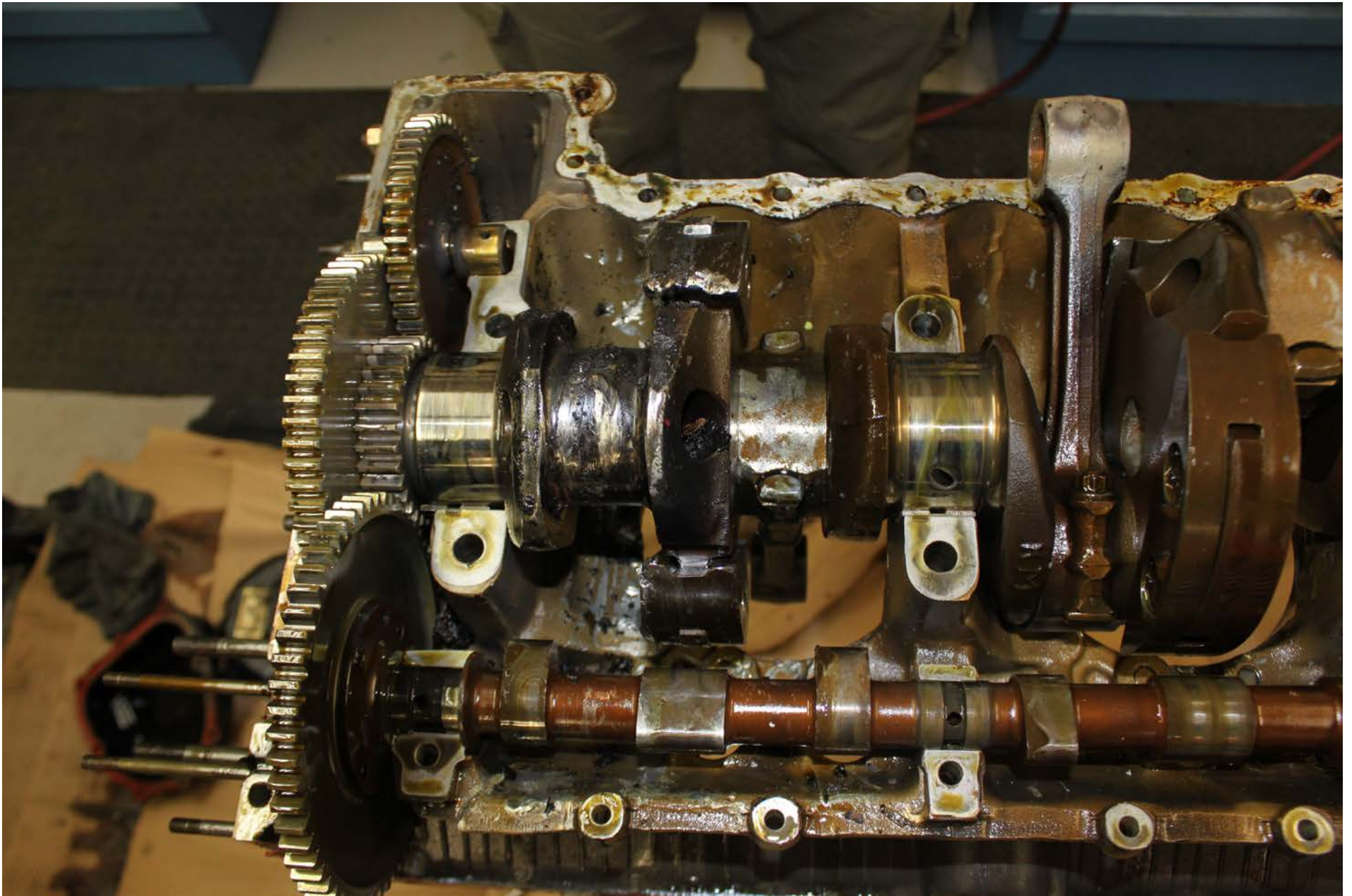
Photo 6 – View of split engine case showing bearing as found on disassembly
