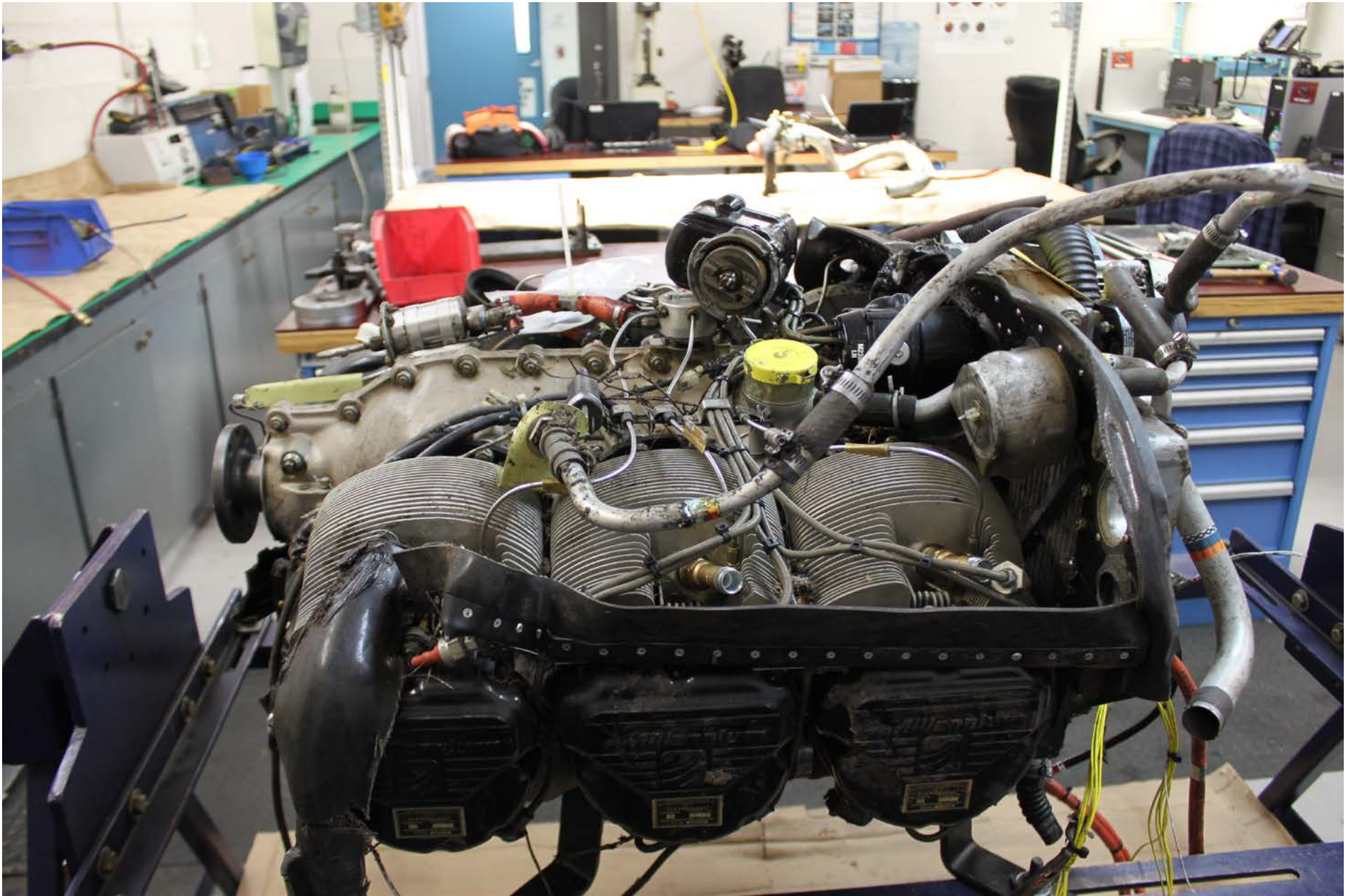
Photo 4 – View of engine during disassembly
