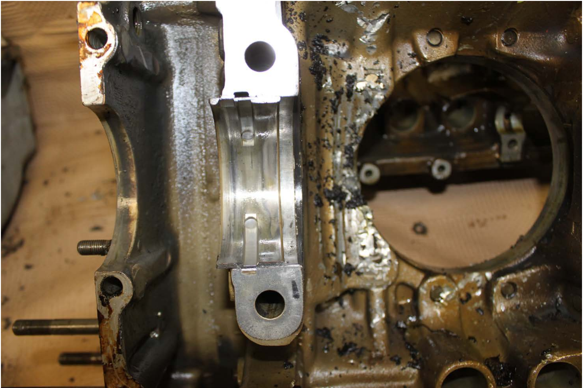
Photo 8 – Close of up shifted bearing after crankshaft removal
