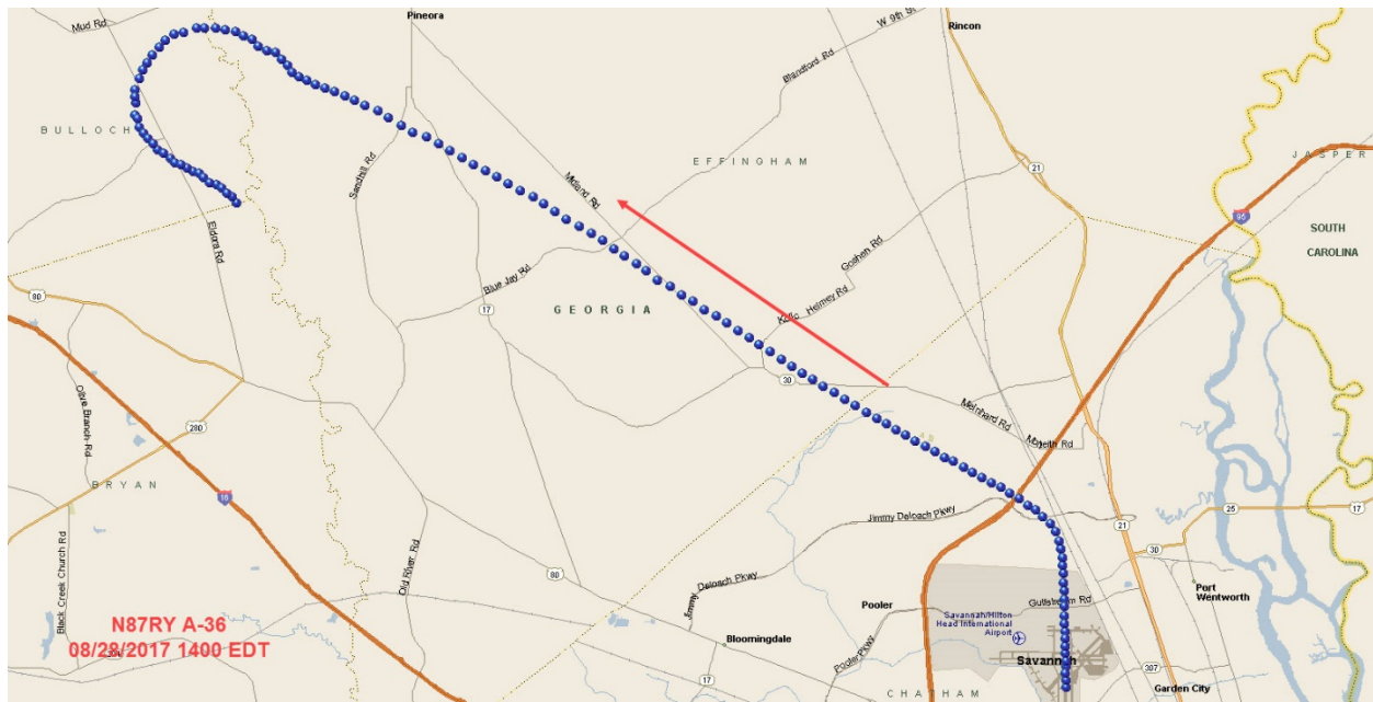
Figure 2- Plot of entire flight path
