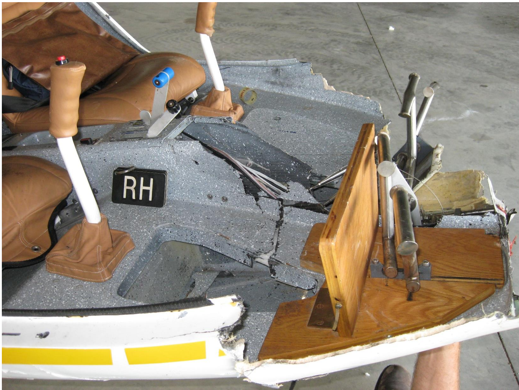
Photo 6 – Overview of Rudder Pedal Guard Device
