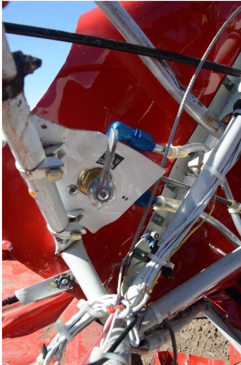
Photo 8 - View of the 5-gallon wing tank shut off valve.
