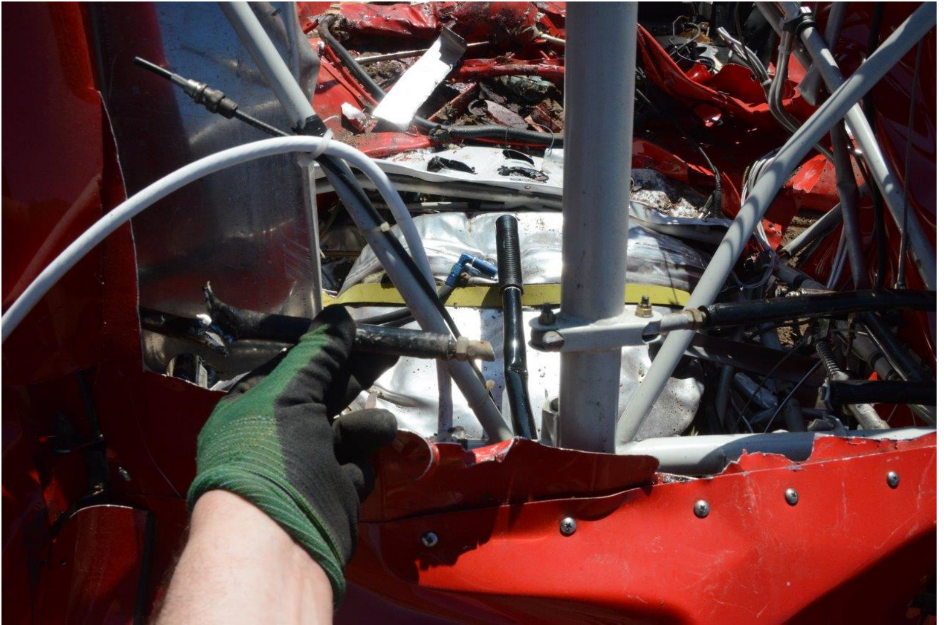
Photo 12 - View of separations in a push pull tube.
