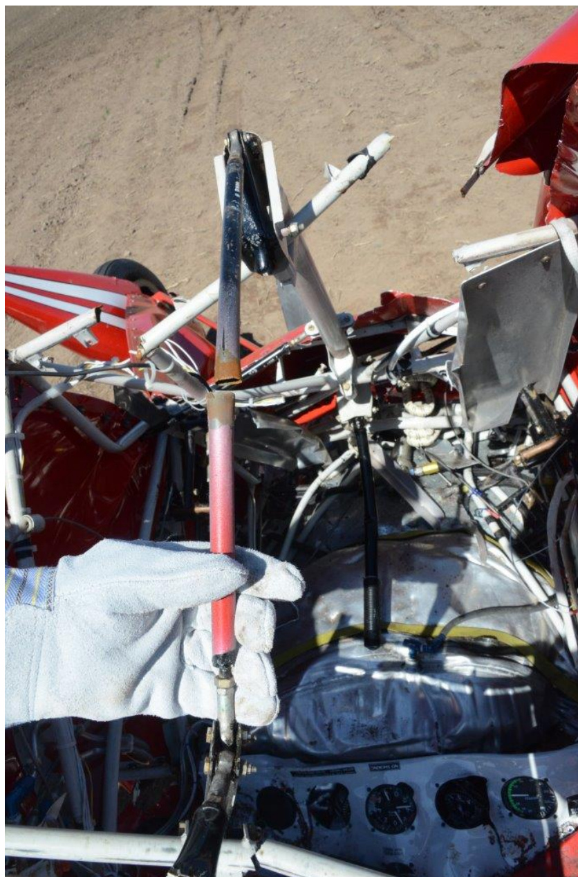
Photo 7 - View of separations in the push pull tubes.
