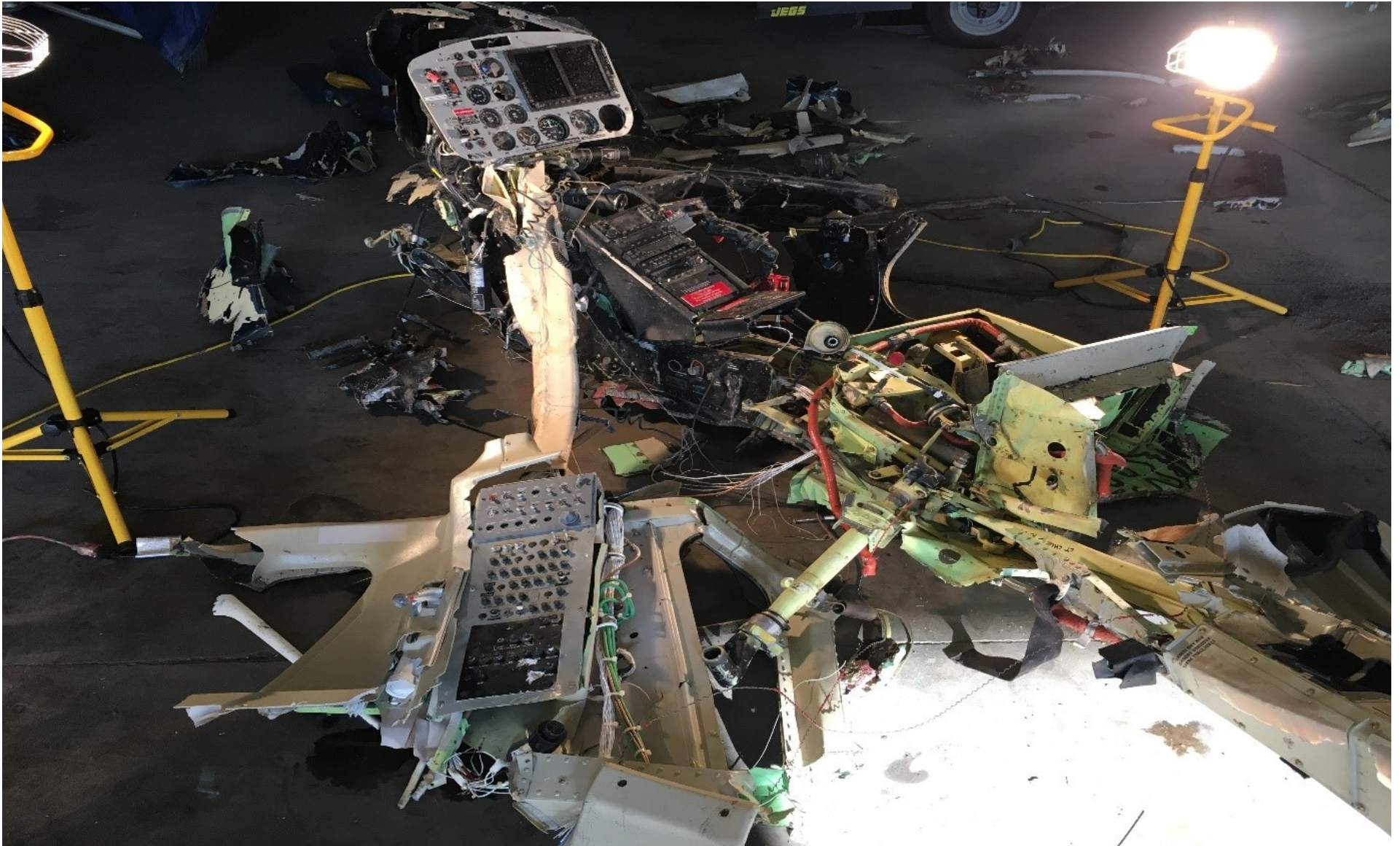
Photo 4 - Closeup of Helicopter Wreckage Cockpit Section
