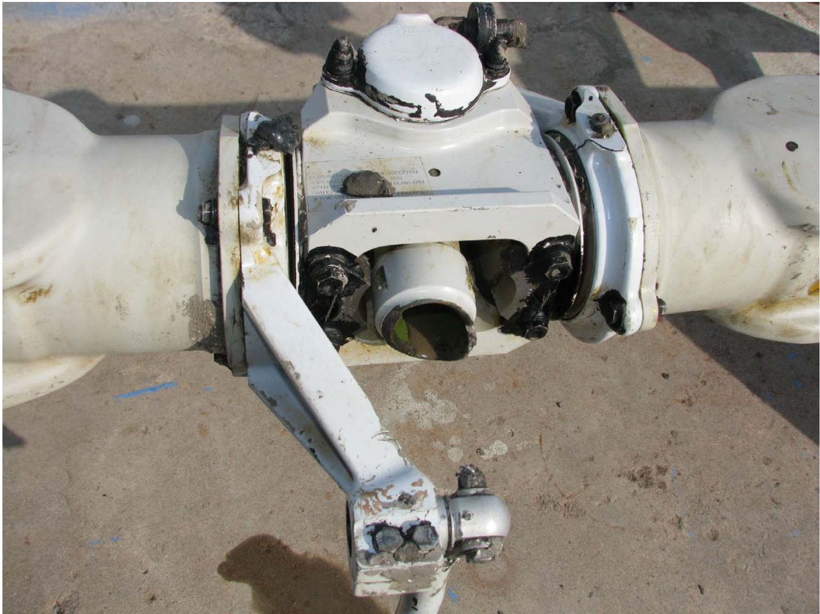
Photo 8 – Main rotor hub bore evidence of torsional overload and mast rubbing.
