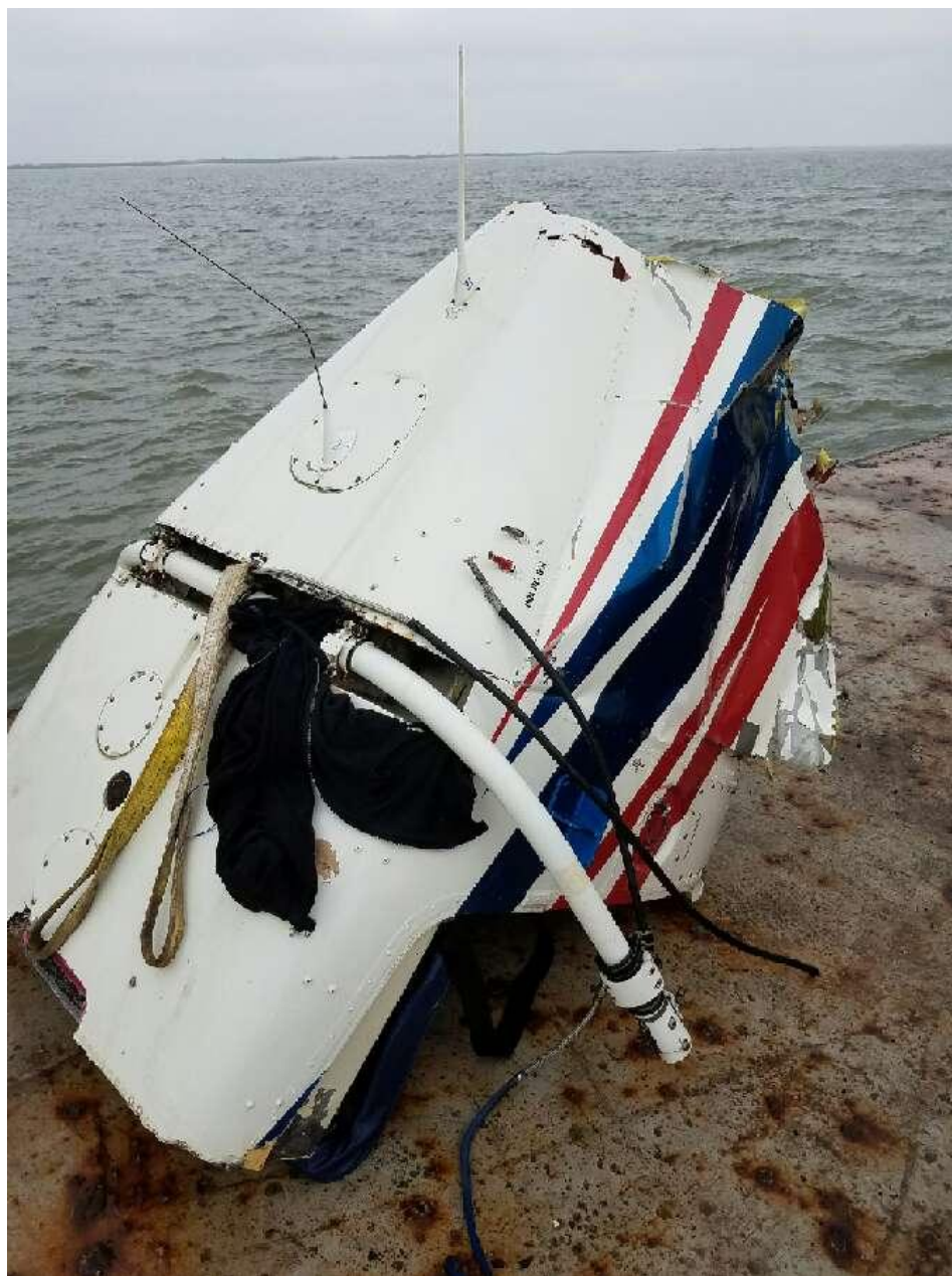
Photo 2 – Bottom portion of fuselage and landing skid after recovery from West Bay.
