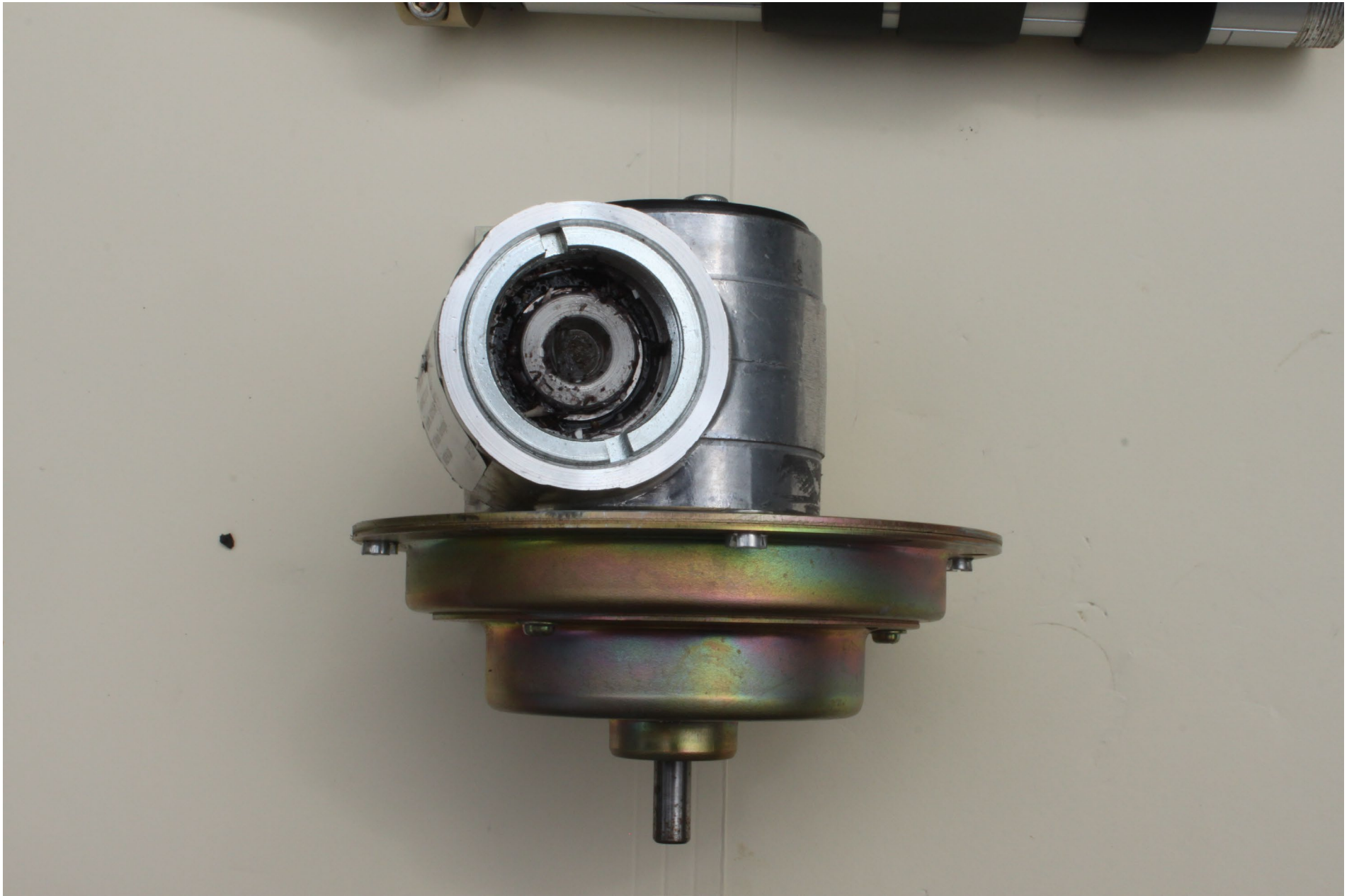
Photo 10 – Flap Actuator
