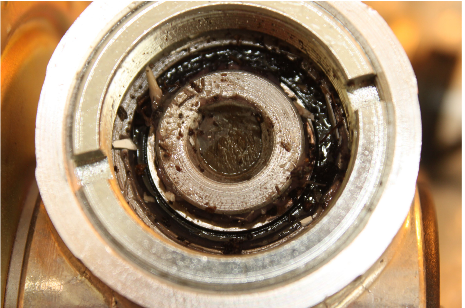
Photo 12 – Flap Actuator
