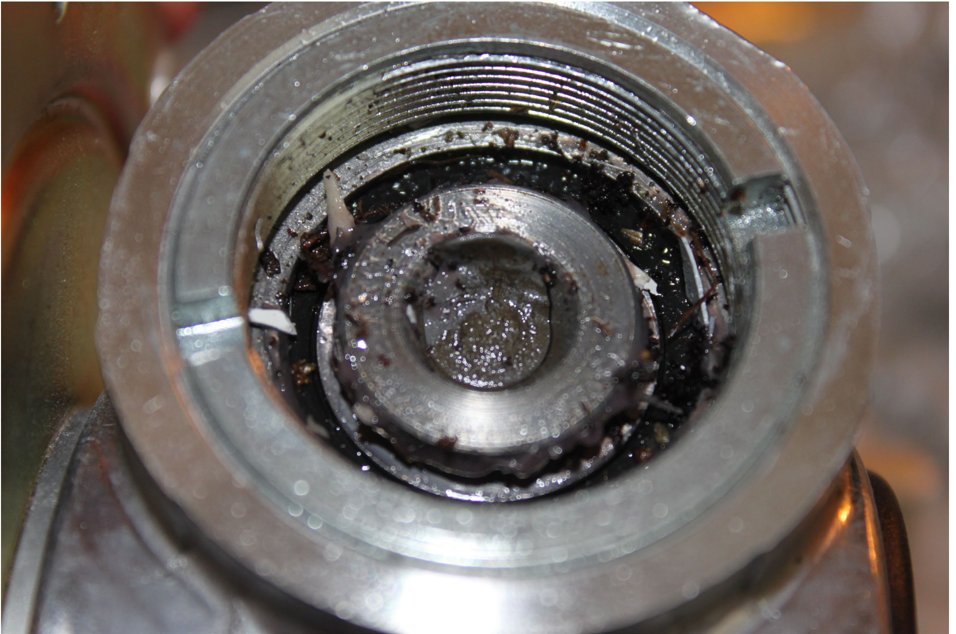
Photo 16 – Flap Actuator
