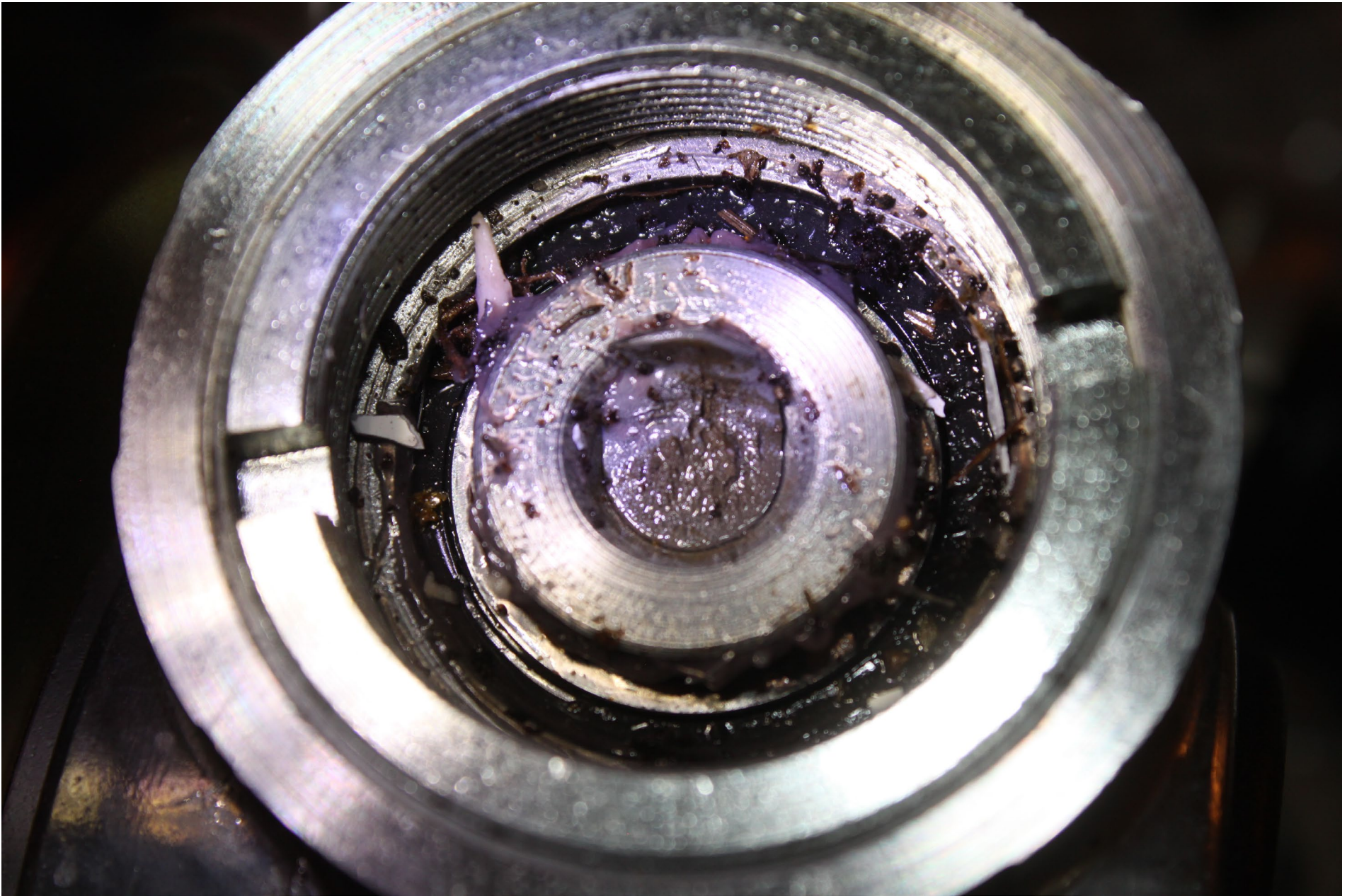
Photo 13 – Flap Actuator
