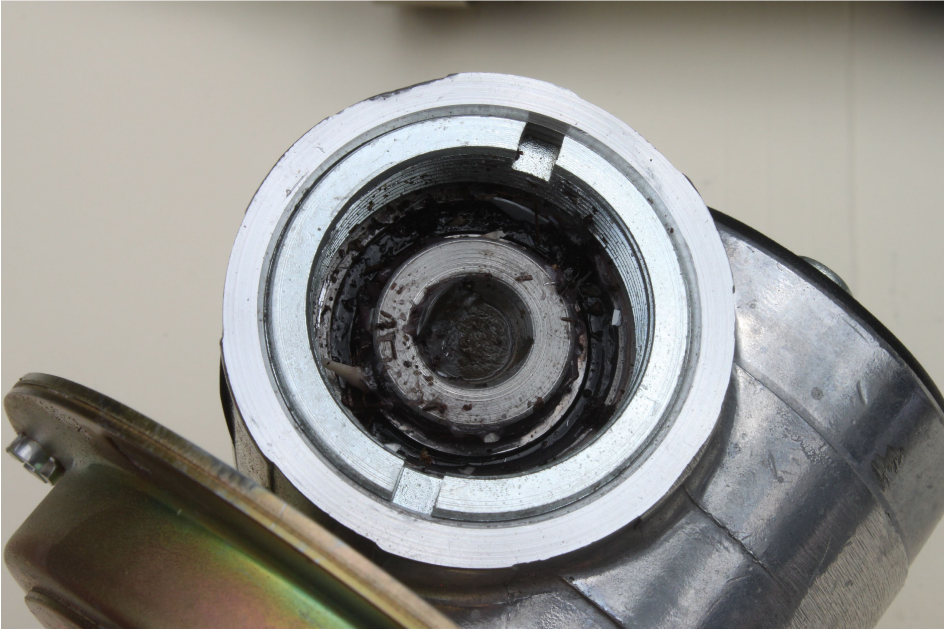
Photo 11 – Flap Actuator
