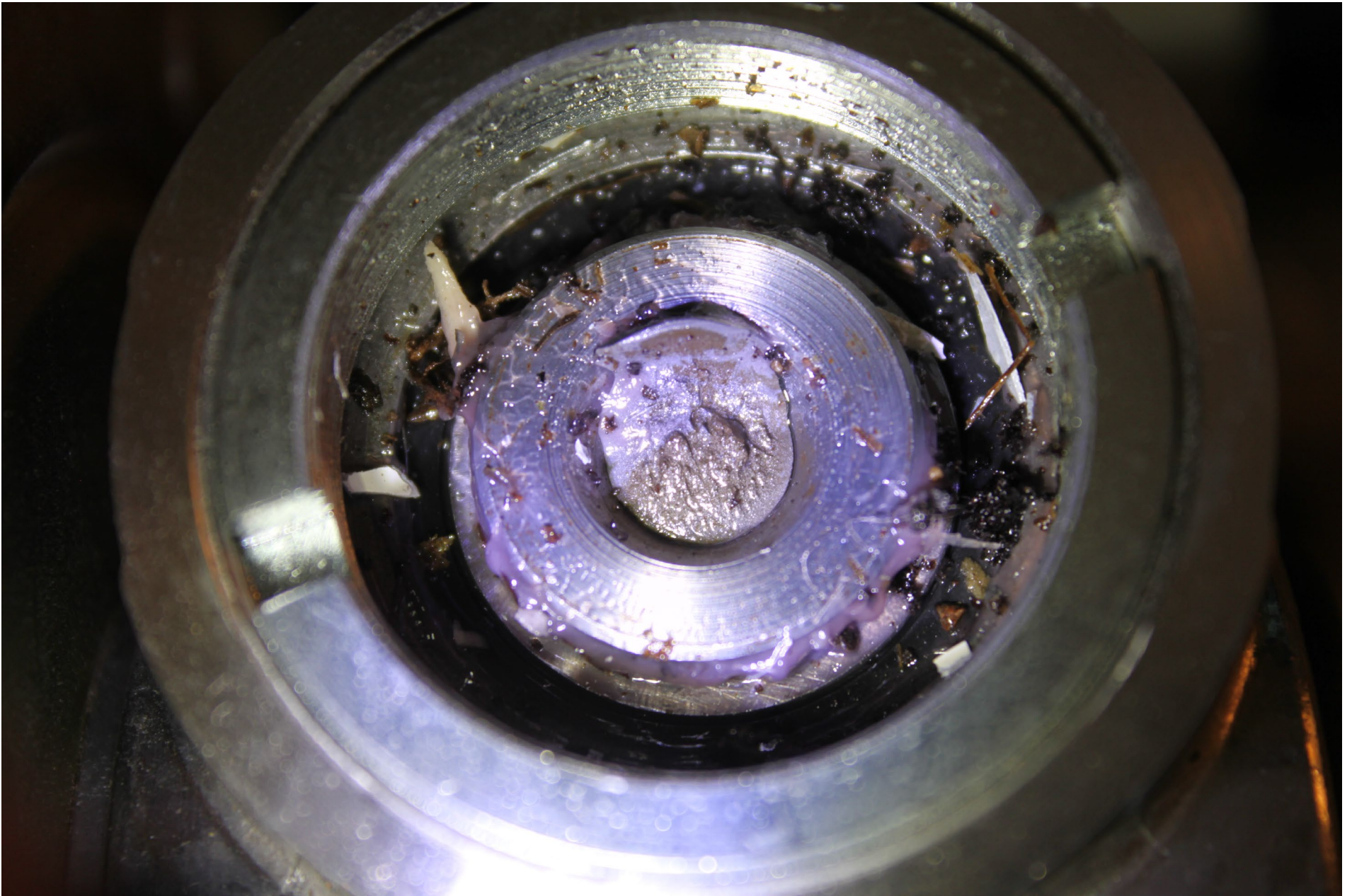
Photo 18 – Flap Actuator
