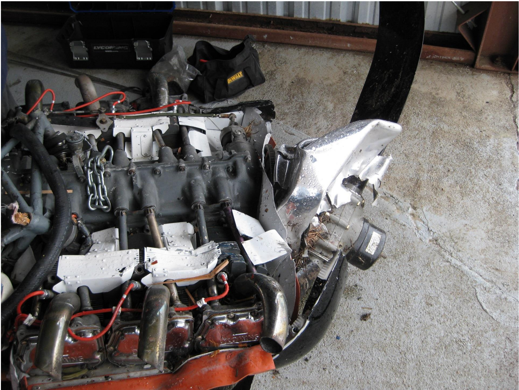
Photo 16 – View of the top of the engine and propeller
