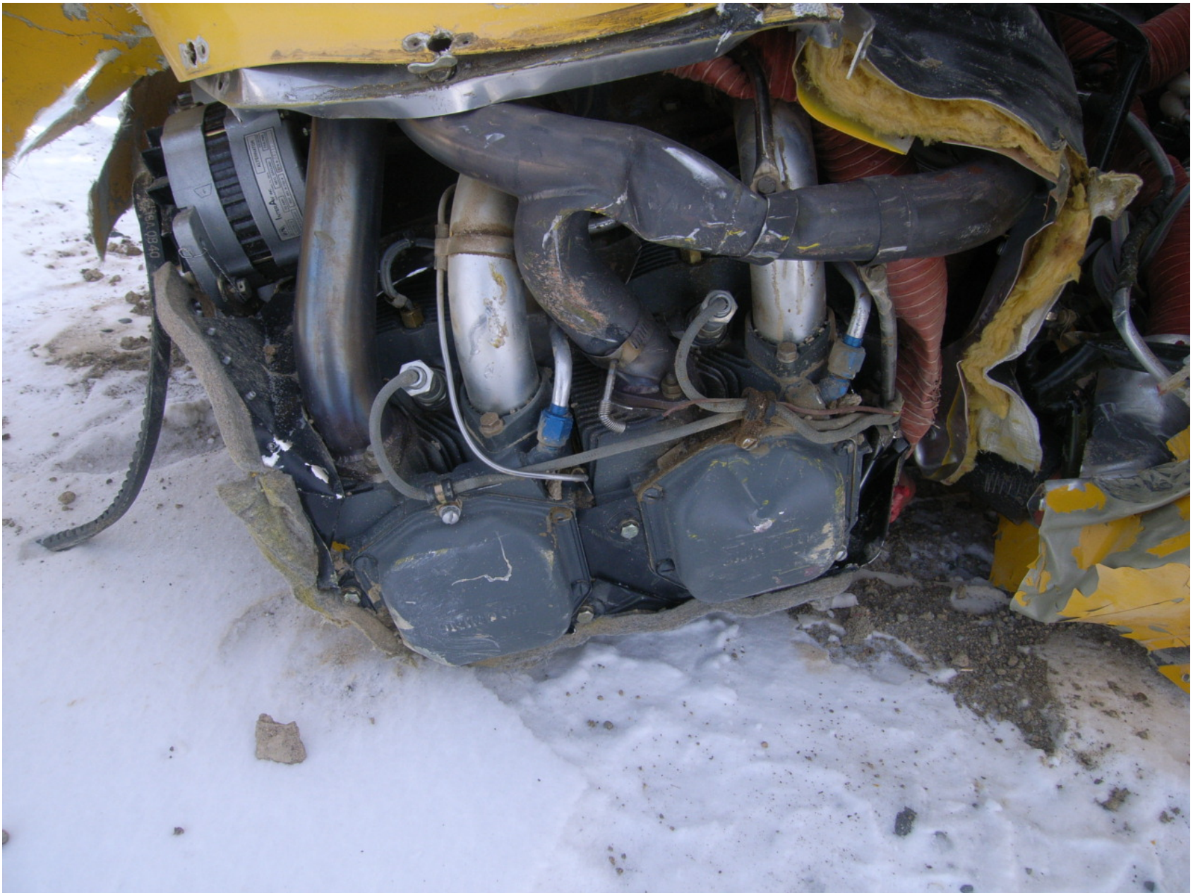
Photograph 7 - Engine
