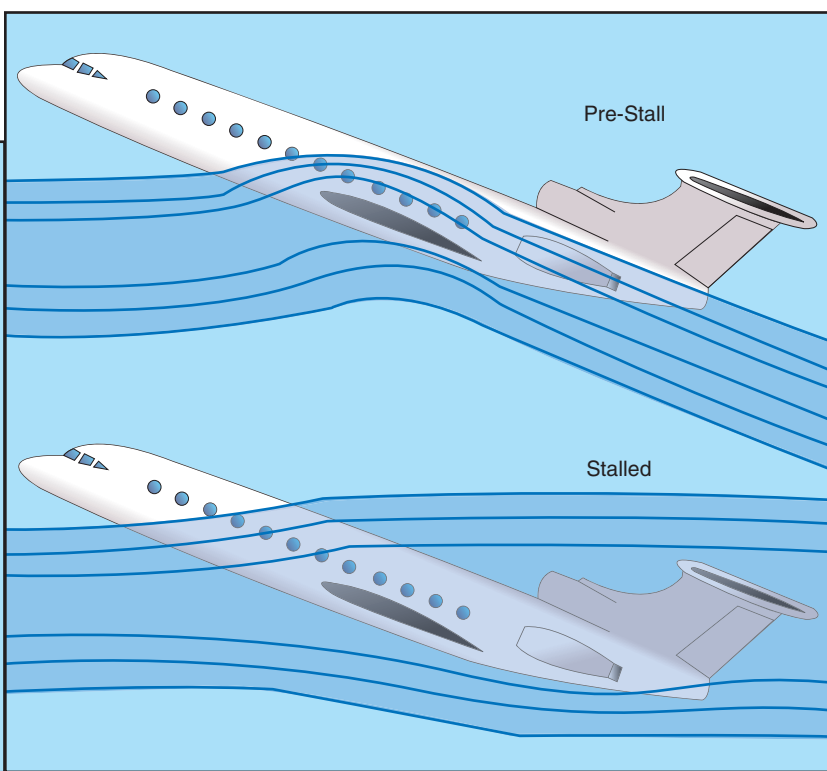
Figure 3-46. T-tail stall.
