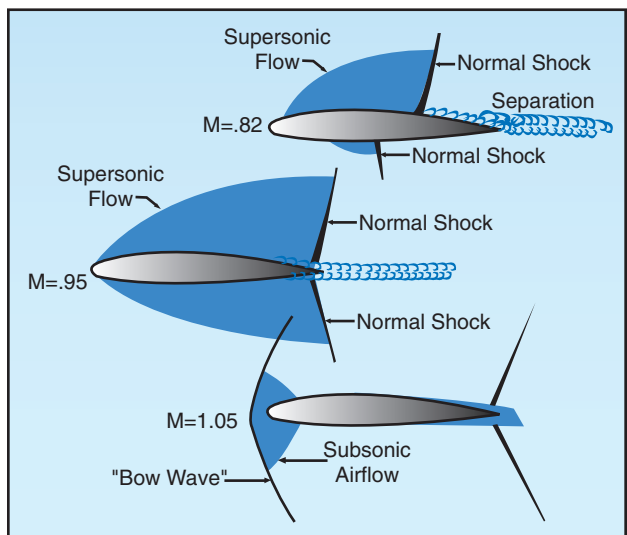
Figure 3-43. Shock waves.
