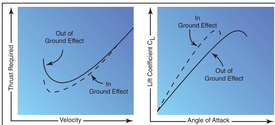
Figure 3-8. Ground effect changes drag and lift.
