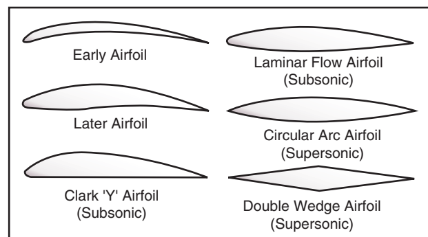
Figure 2-6. Airfoil designs.
