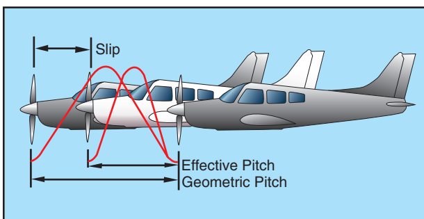
Figure 3-28. Propeller slippage.
