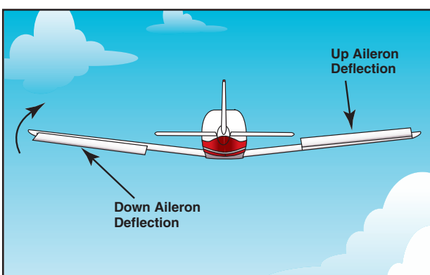
Figure 4-3. Differential ailerons.
