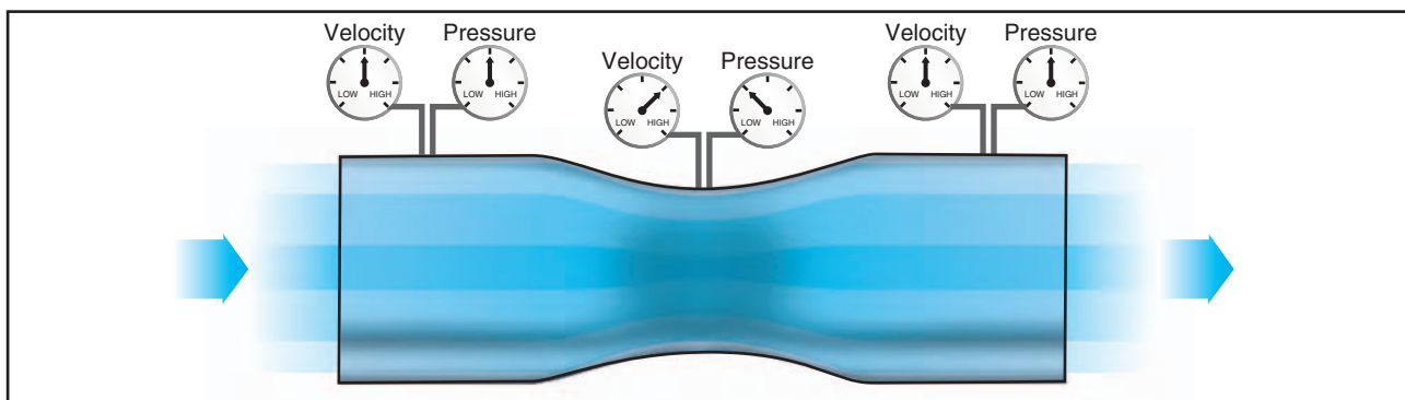
Figure 2-4. Air pressure decreases in a venturi.
