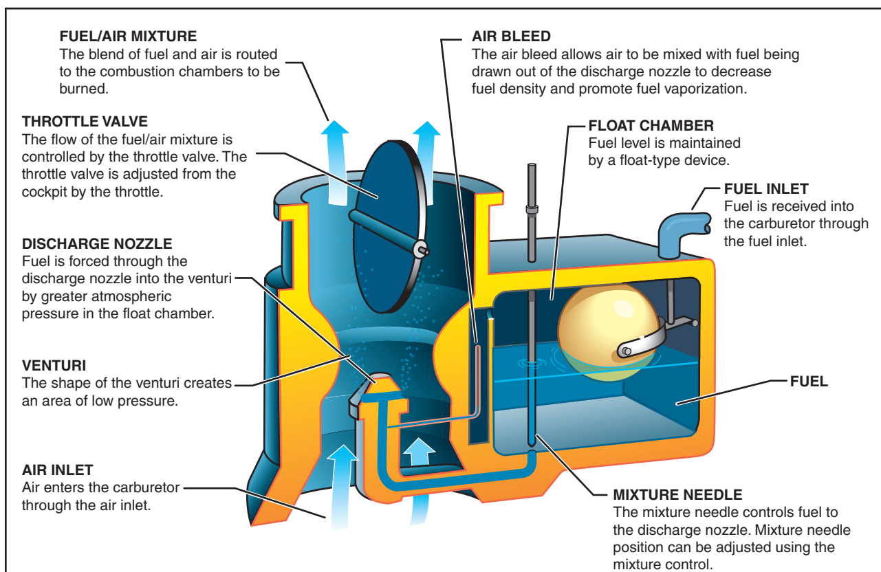
Figure 5-7. Float-type carburetor.
