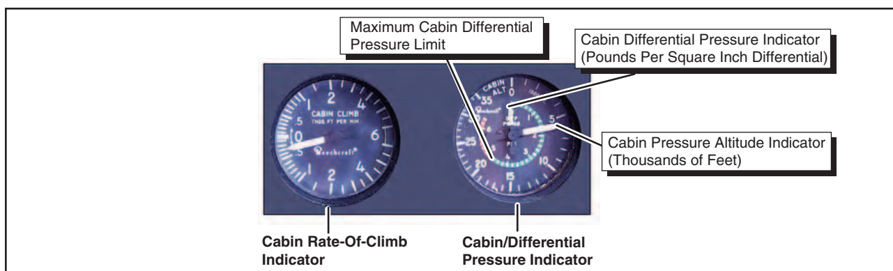
Figure 5-31. Cabin pressurization instruments.
