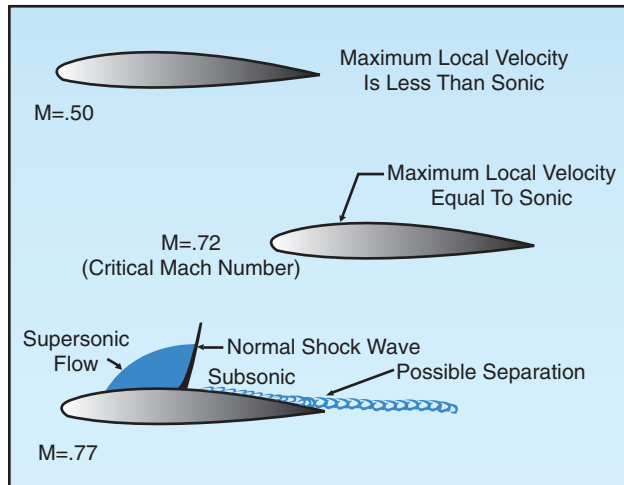
Figure 3-40. Wing airflow.
