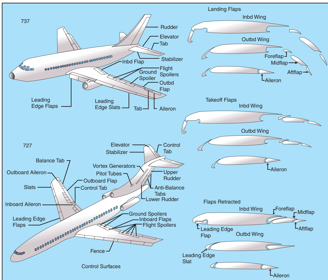
Figure 3-47. Control surfaces.
