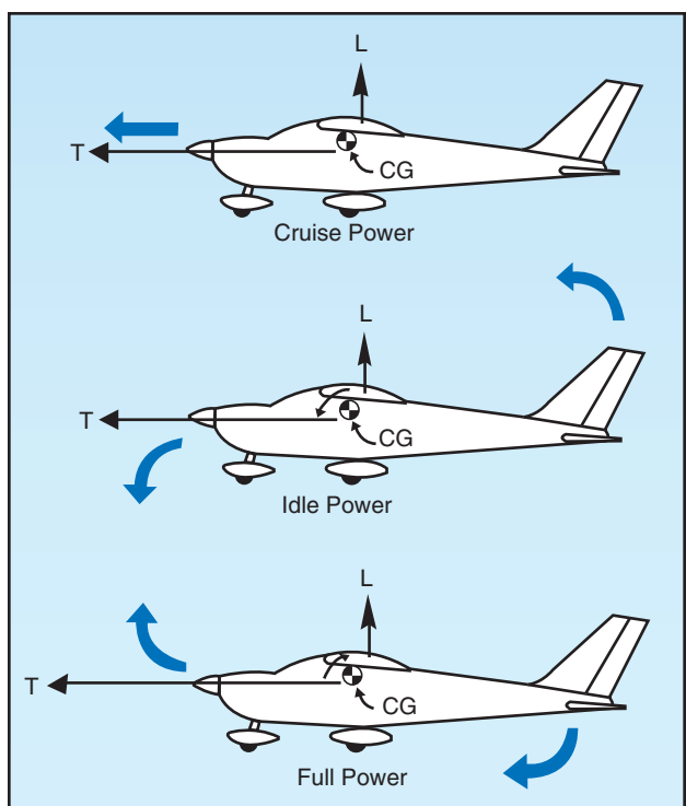
Figure 3-16. Power changes affect longitudinal stability.
