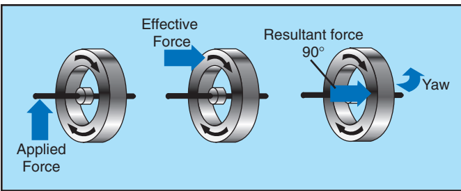
Figure 3-32. Gyroscopic precession.
