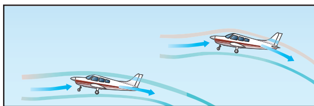
Figure 3-7. Ground effect changes airflow.
