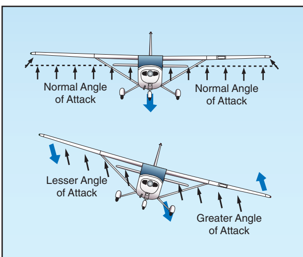
Figure 3-17. Dihedral for lateral stability.
