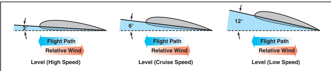
Figure 3-3. Angle of attack at various speeds.
