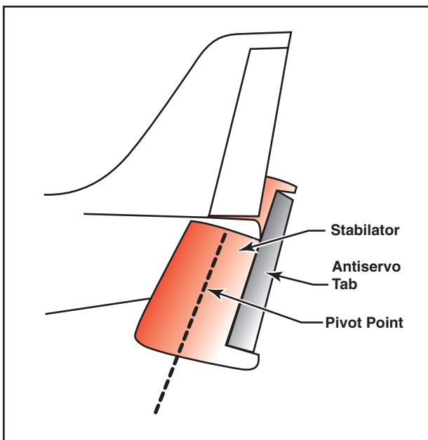
Figure 1-8. Stabilator components.
