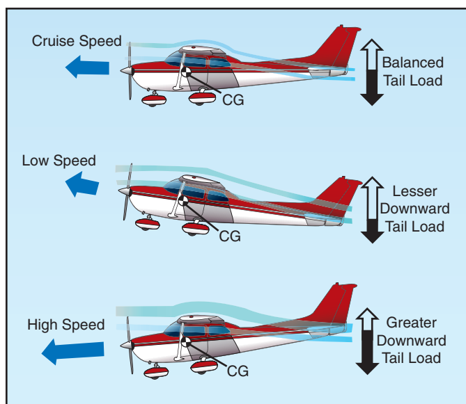
Figure 3-13. Effect of speed on downwash.
