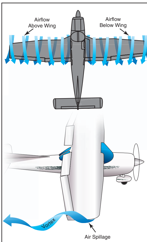
Figure 3-4. Wingtip vortices.
