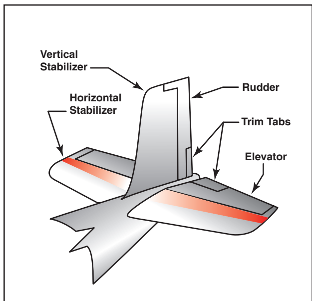
Figure 1-7. Empennage components.
