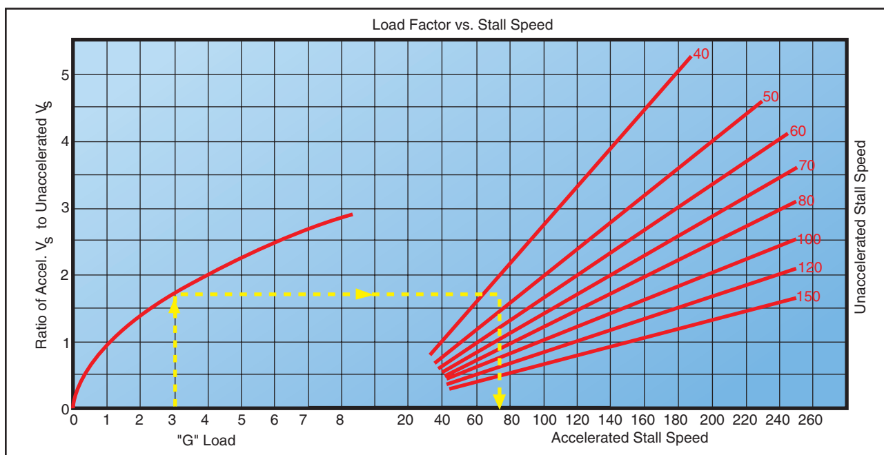
Figure 3-37. Load factor changes stall speed.
