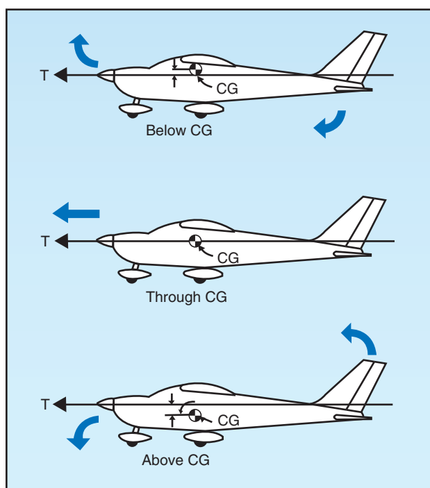
Figure 3-15. Thrust line affects longitudinal stability.
