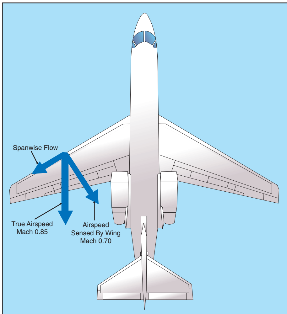
Figure 3-44. Sweepback effect.
