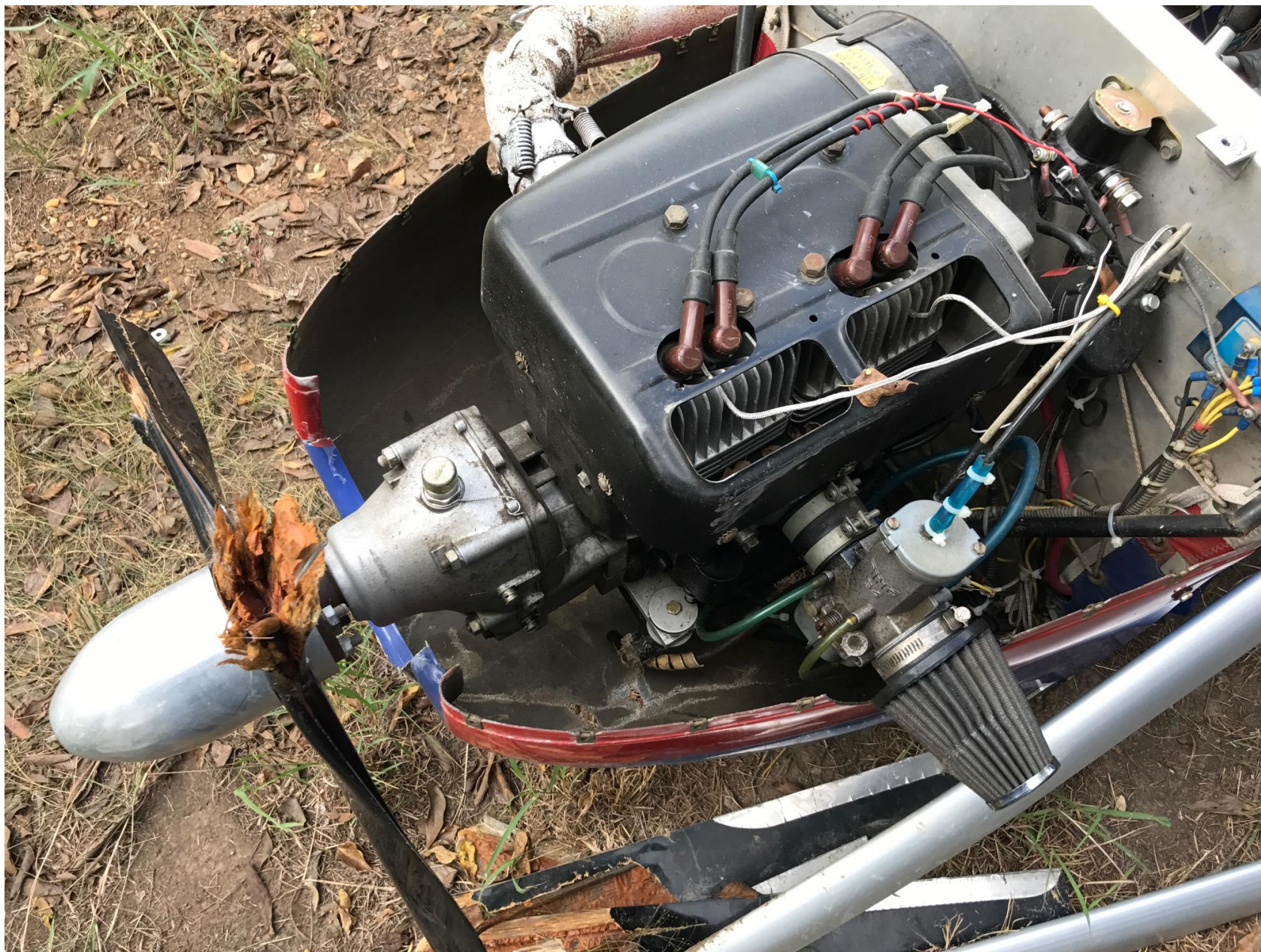
Photo 3 – Engine (FAA Photo)
