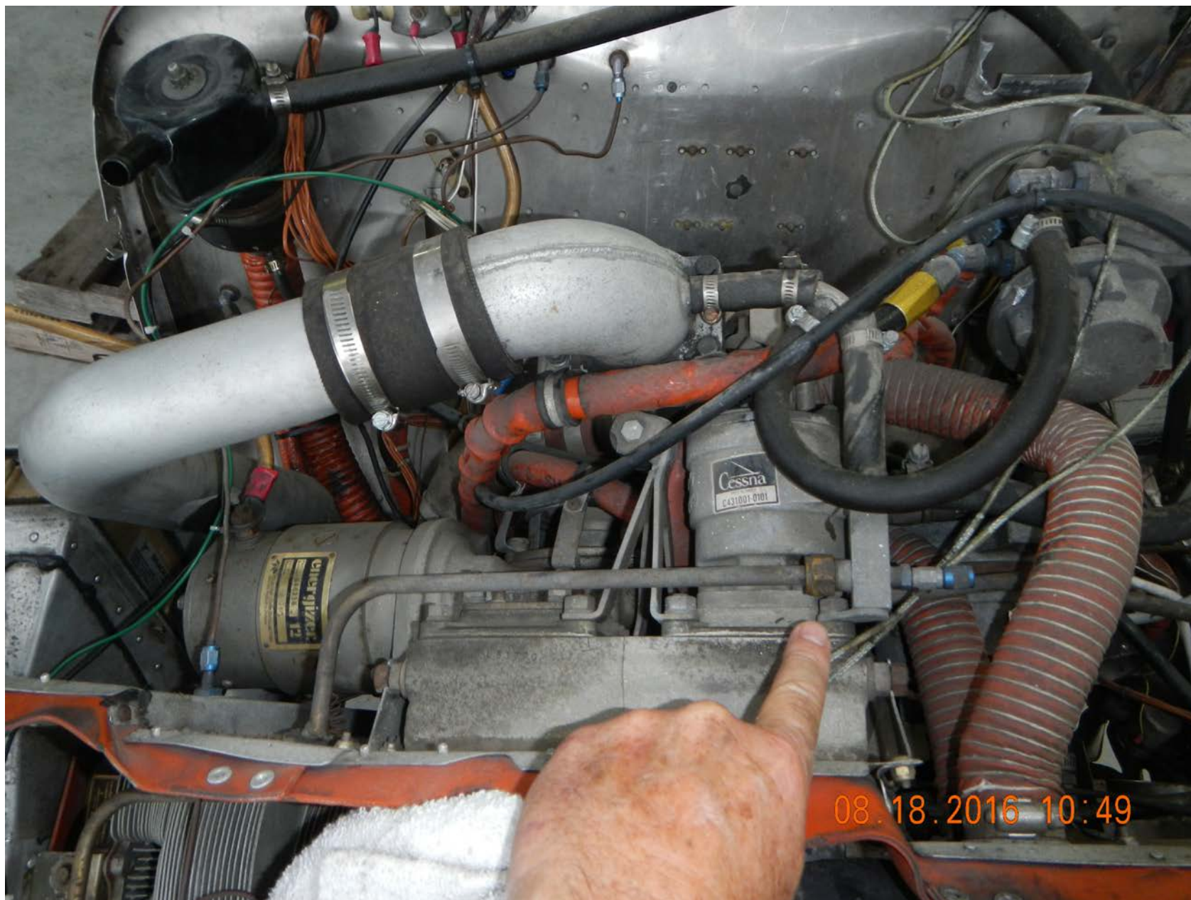
Photo 5 - Loose B-Nut Fitting Observed During Engine Examination
