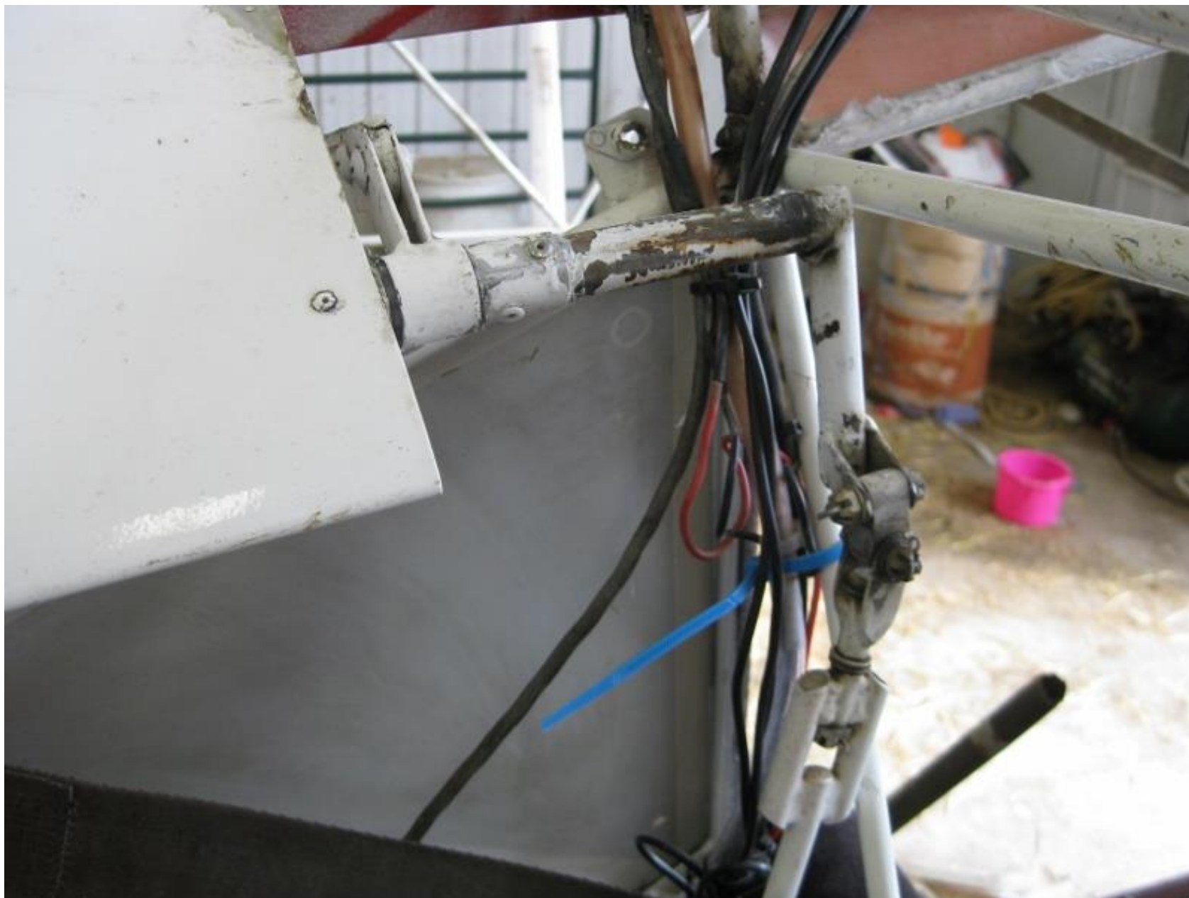
Photo 17 – View of the flaperon control tube and control arm
