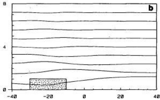
Figure 1. Model of flow past a heat source, from Lin and Smith 1986.
