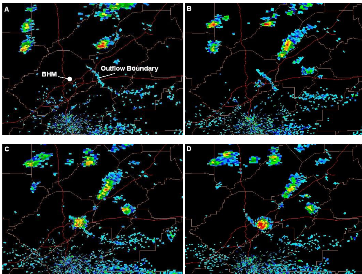
Figure 9. 0.5 degree elevation reflectivity from KBMX WSR-88D radar at a) 0000 UTC; b) 0020 UTC; c) 0032 UTC; and d) 0041 UTC.
