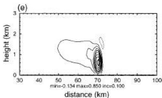
Figure 2. Perturbation vertical velocity associated with urban heat island located at x=50 km, at time t=4 h.
