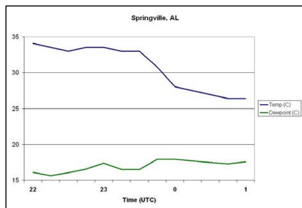
Figure 7. Temperature (blue) and dewpoint (green) (in degrees C) from Springville, AL. Note the drop in temperature at rise in dewpoint with passage of the outflow boundary just after 2330 UTC.
