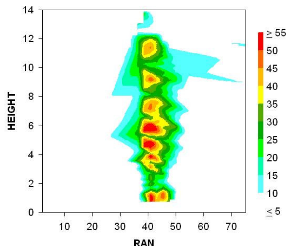
Figure 8. Reflectivity cross-section from KBMX at 10 degrees azimuth, 0032 UTC.
