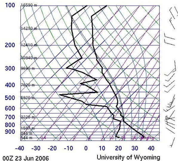
Figure 3. 00 UTC 23 June 2006 sounding at Calera, AL.
