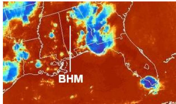
Figure 4. GOES infrared satellite image at 00 UTC 23 Jun 06. Note apparent maximum in brightness temperature near Birmingham. (NCAR)
