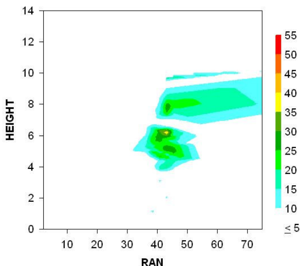
Figure 6. Reflectivity cross-section from KBMX radar at 10 degrees azimuth, 0015 UTC.
