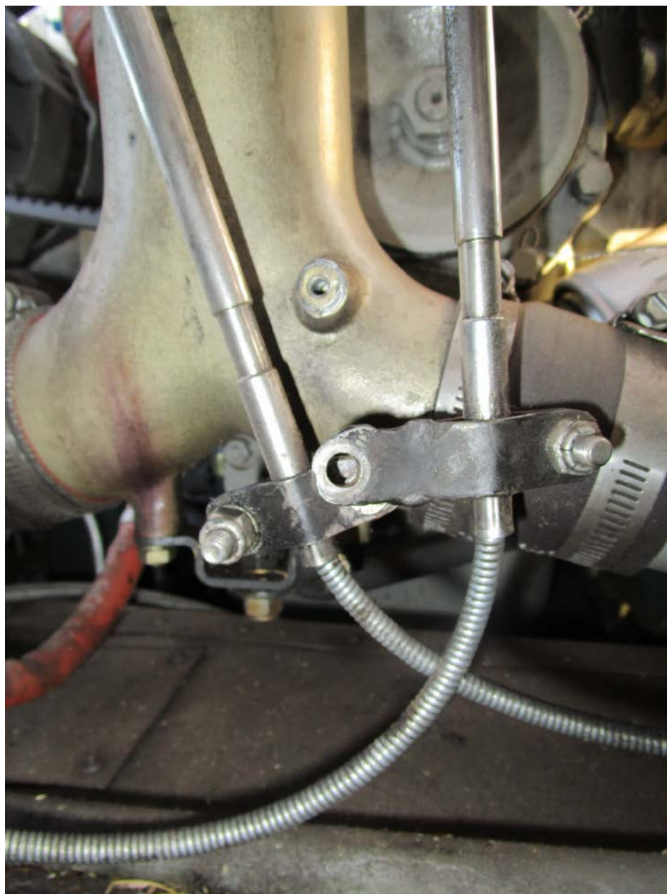
Photo 1 – Loose Bracket
