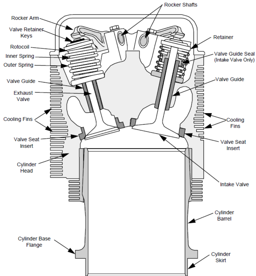
Cylinder Assembly Description IO-520-B, -BA, -BB, -C, -CB, -M, -MB
