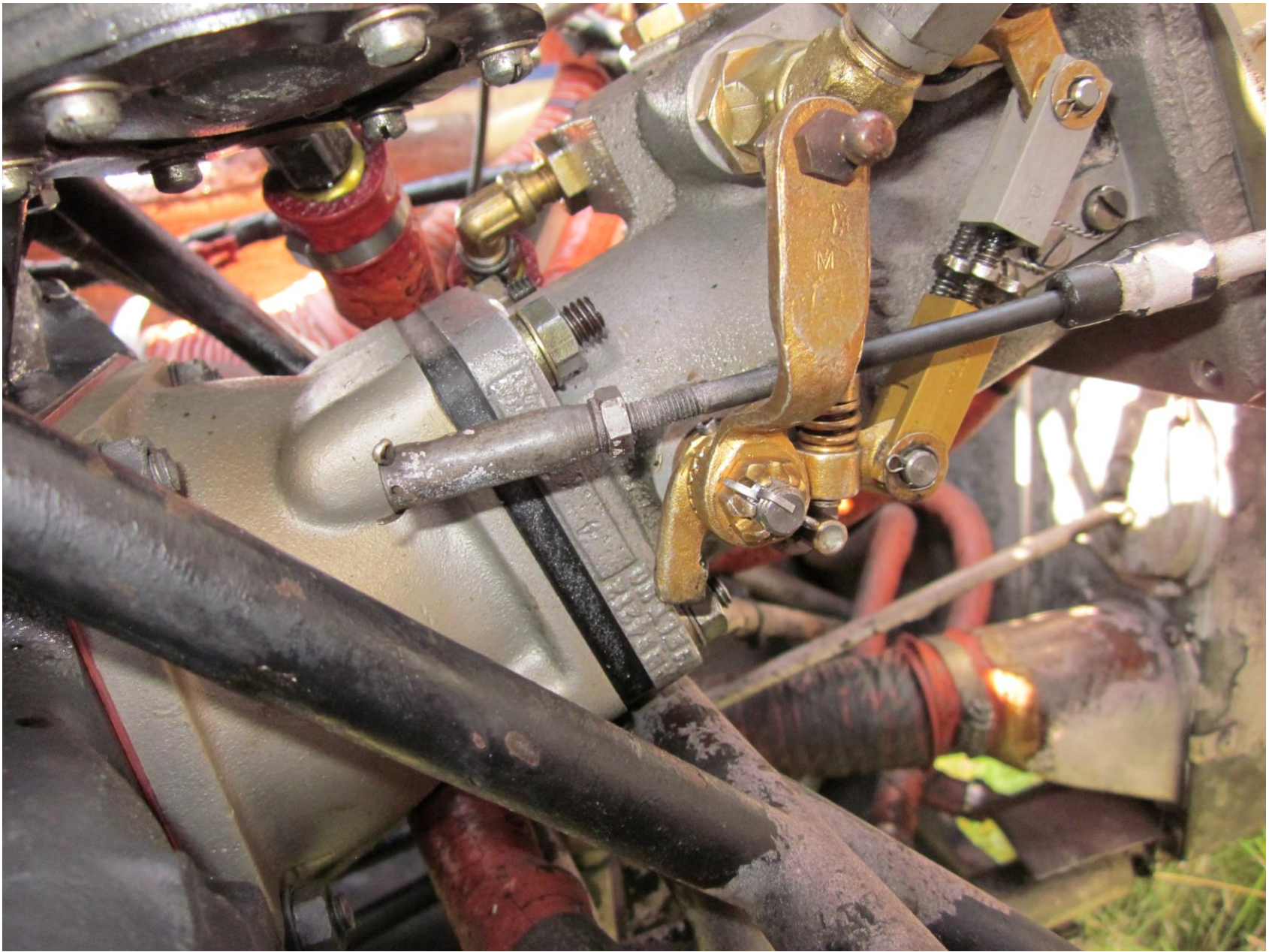
Photo 1 – Separated Throttle Control Arm
