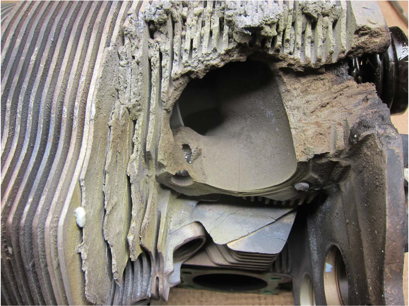
Photo 2 – View of Number 4 Cylinder
