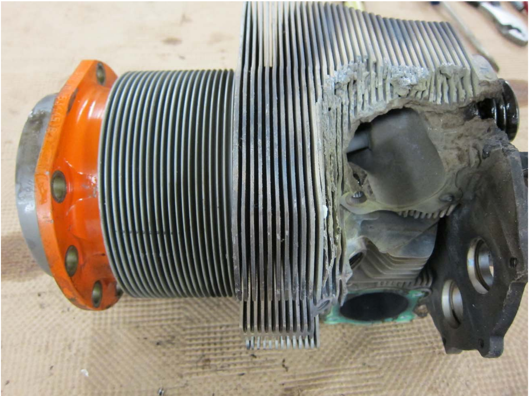
Photo 1 – View of Number 4 Cylinder
