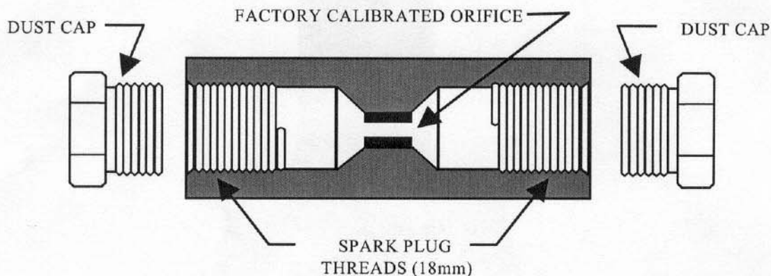
FIGURE 3 MASTER ORIFICE P/N 646953
